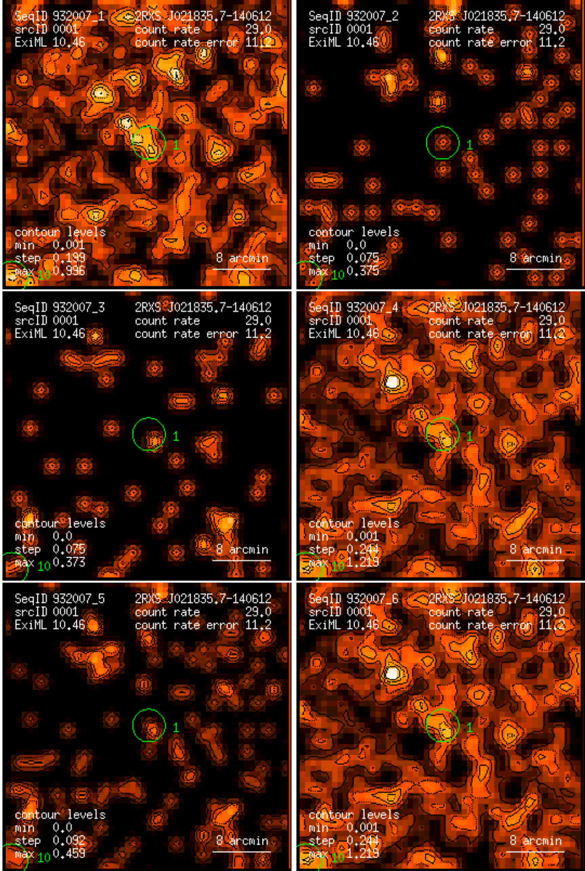
Figure 1: RASS 932007: detection 0001: band rate images, Gaussian filter: (1) PSPC channels 11 – 41, (2) 52 – 90, (3) 91 – 201, (4) 11 – 235, (5) 52 – 201, (6) 11 – 201. Broad band rates in counts/ks. Band rate contour levels in counts/ks/arcmin 2 .
