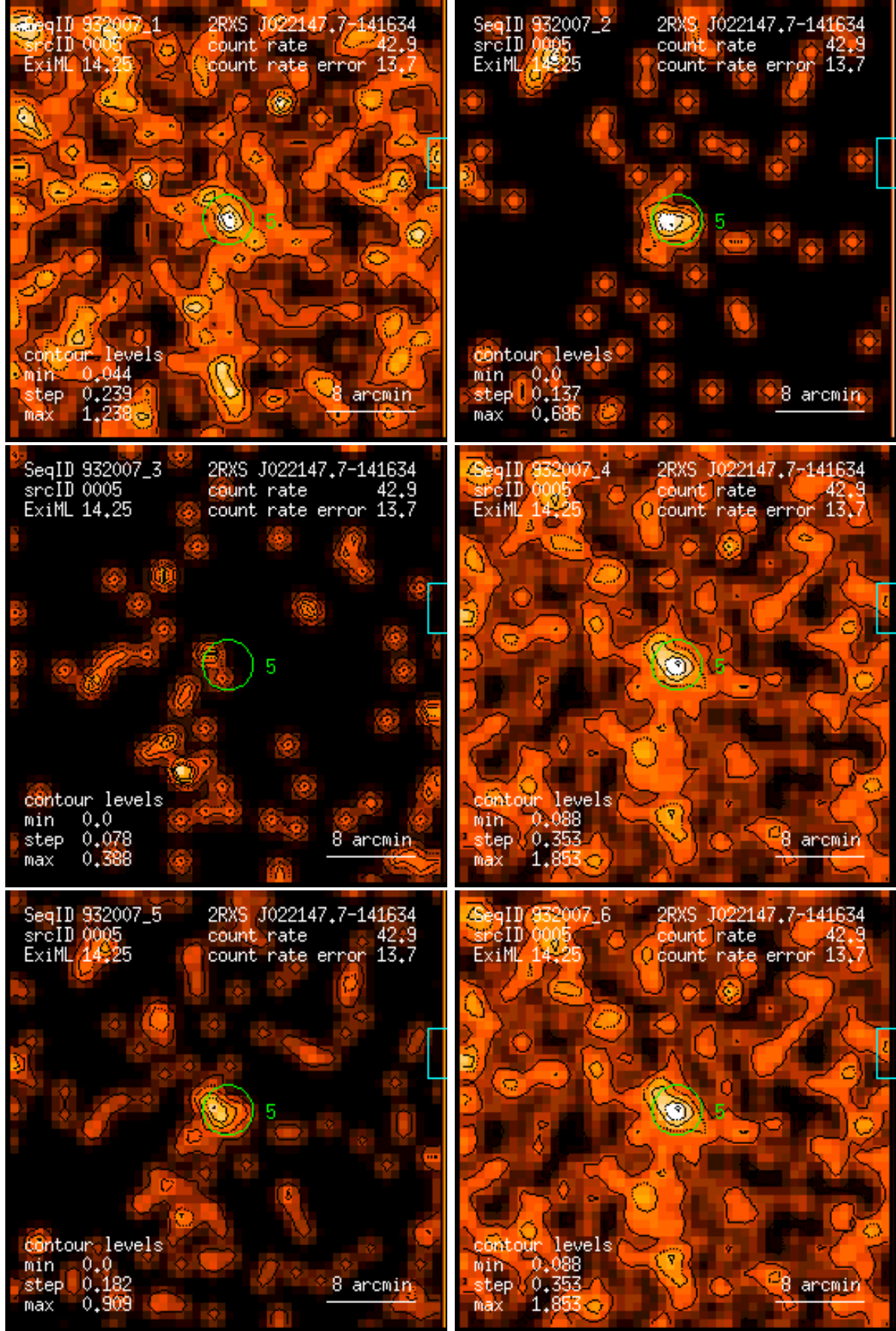
Figure 5: RASS 932007: detection 0005: band rate images, Gaussian filter: (1) PSPC channels 11 – 41, (2) 52 – 90, (3) 91 – 201, (4) 11 – 235, (5) 52 – 201, (6) 11 – 201. Broad band rates in counts/ks. Band rate contour levels in counts/ks/arcmin 2 .
