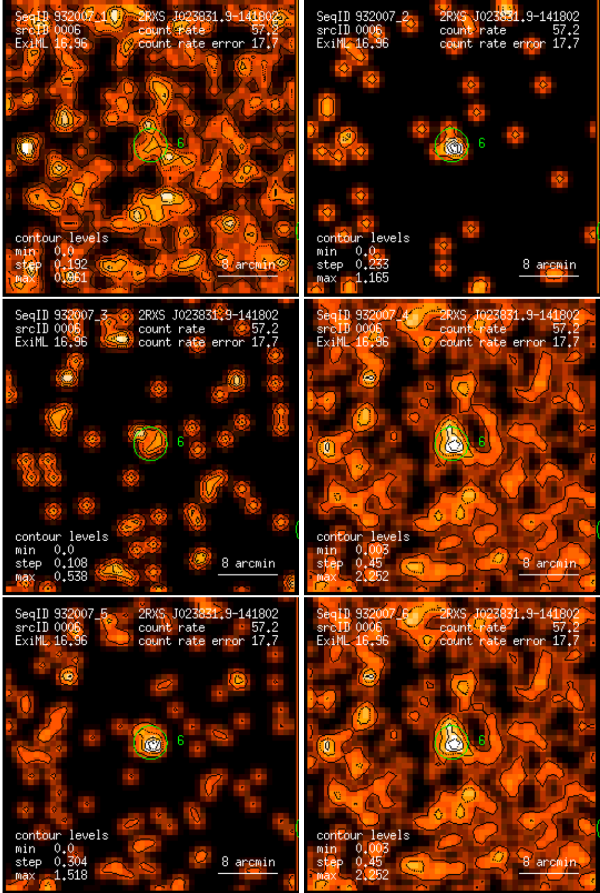
Figure 6: RASS 932007: detection 0006: band rate images, Gaussian filter: (1) PSPC channels 11 – 41, (2) 52 – 90, (3) 91 – 201, (4) 11 – 235, (5) 52 – 201, (6) 11 – 201. Broad band rates in counts/ks. Band rate contour levels in counts/ks/arcmin 2 .
