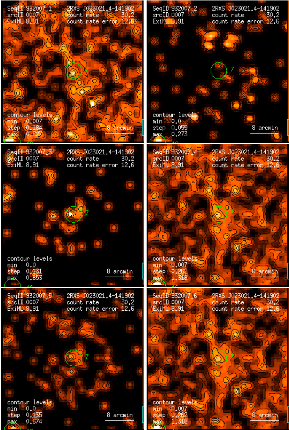
Figure 7: RASS 932007: detection 0007: band rate images, Gaussian filter: (1) PSPC channels 11 – 41, (2) 52 – 90, (3) 91 – 201, (4) 11 – 235, (5) 52 – 201, (6) 11 – 201. Broad band rates in counts/ks. Band rate contour levels in counts/ks/arcmin 2 .
