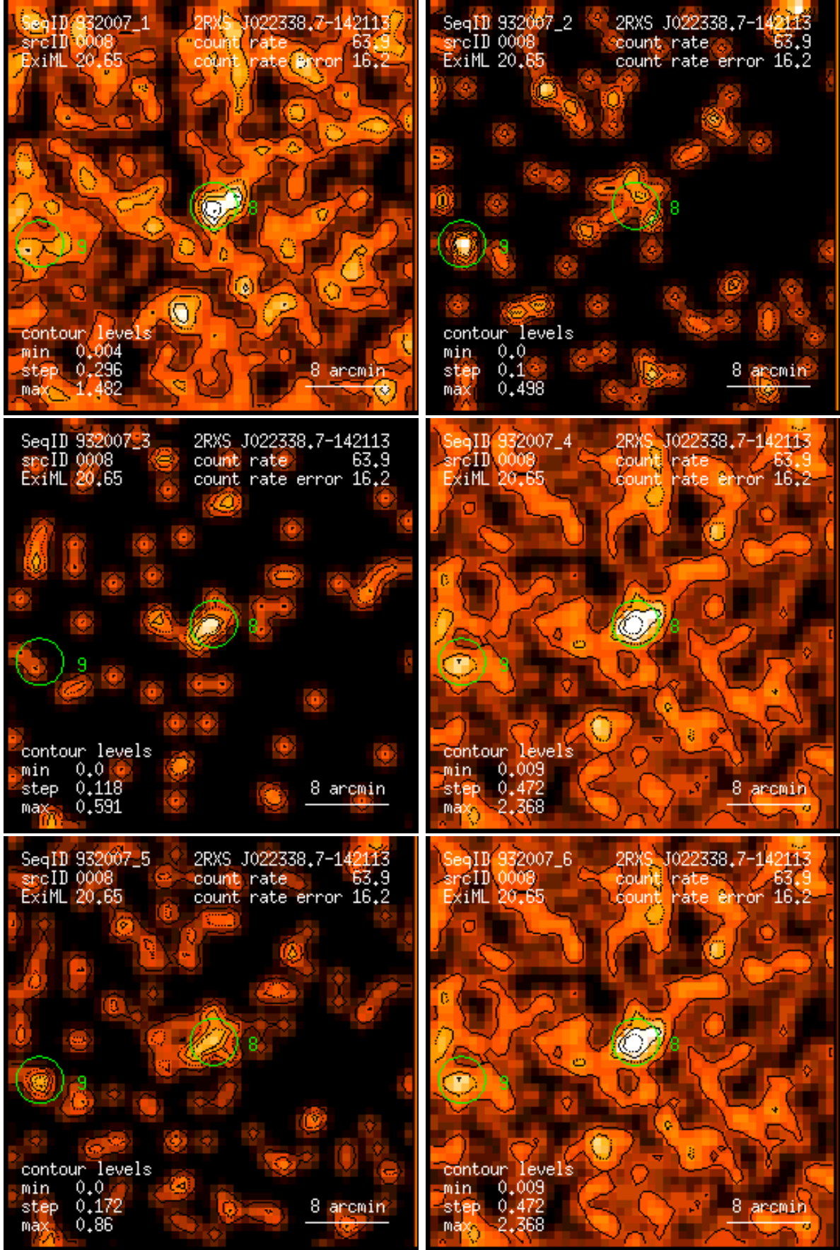
Figure 8: RASS 932007: detection 0008: band rate images, Gaussian filter: (1) PSPC channels 11 – 41, (2) 52 – 90, (3) 91 – 201, (4) 11 – 235, (5) 52 – 201, (6) 11 – 201. Broad band rates in counts/ks. Band rate contour levels in counts/ks/arcmin 2 .
