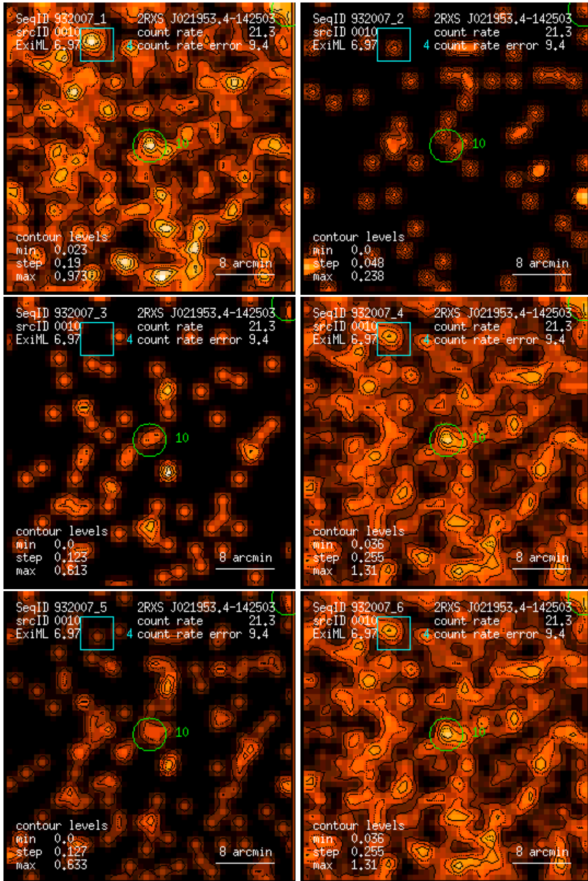
Figure 10: RASS 932007: detection 0010: band rate images, Gaussian filter: (1) PSPC channels 11 – 41, (2) 52 – 90, (3) 91 – 201, (4) 11 – 235, (5) 52 – 201, (6) 11 – 201. Broad band rates in counts/ks. Band rate contour levels in counts/ks/arcmin 2 .
