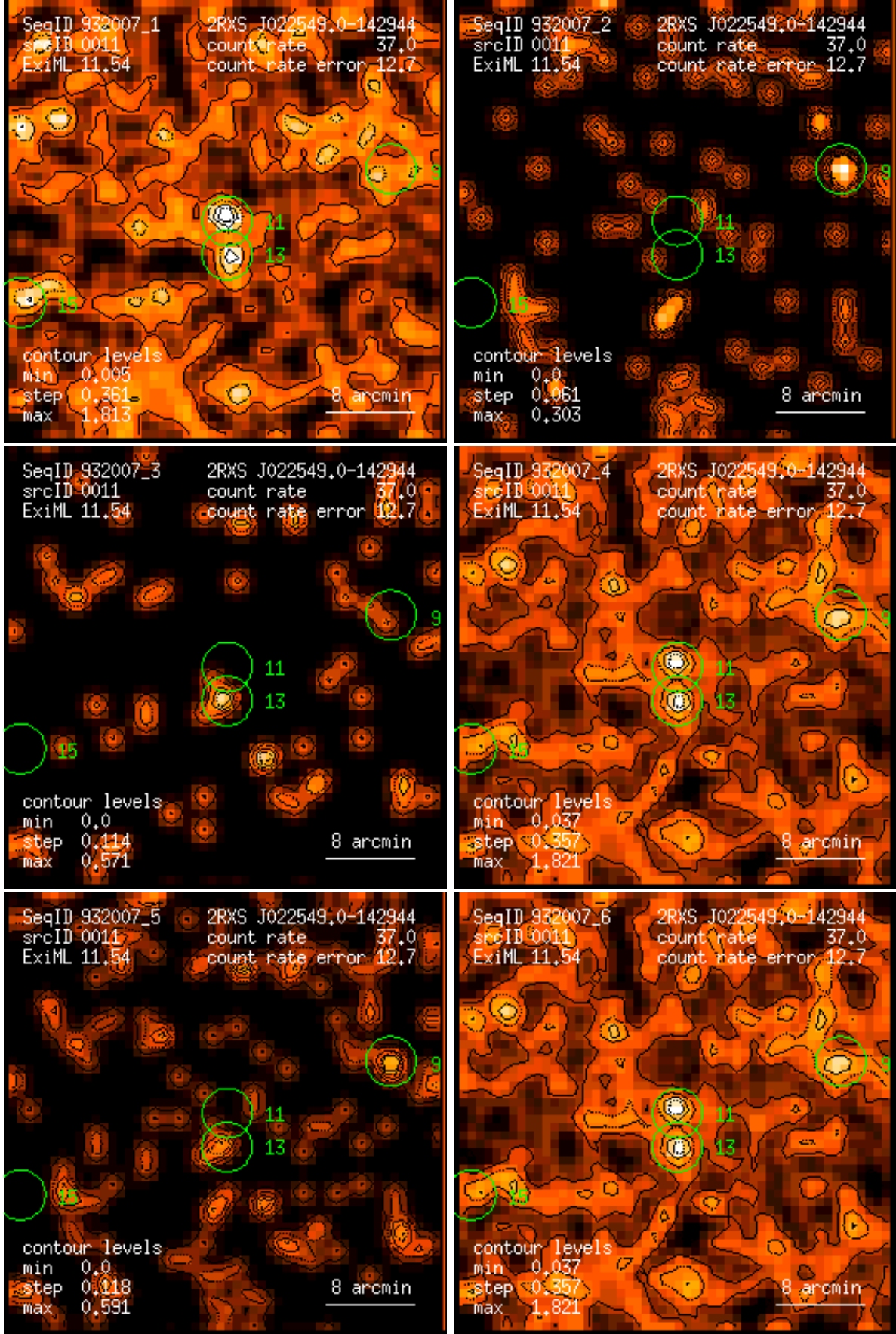
Figure 11: RASS 932007: detection 0011: band rate images, Gaussian filter: (1) PSPC channels 11 – 41, (2) 52 – 90, (3) 91 – 201, (4) 11 – 235, (5) 52 – 201, (6) 11 – 201. Broad band rates in counts/ks. Band rate contour levels in counts/ks/arcmin 2 .
