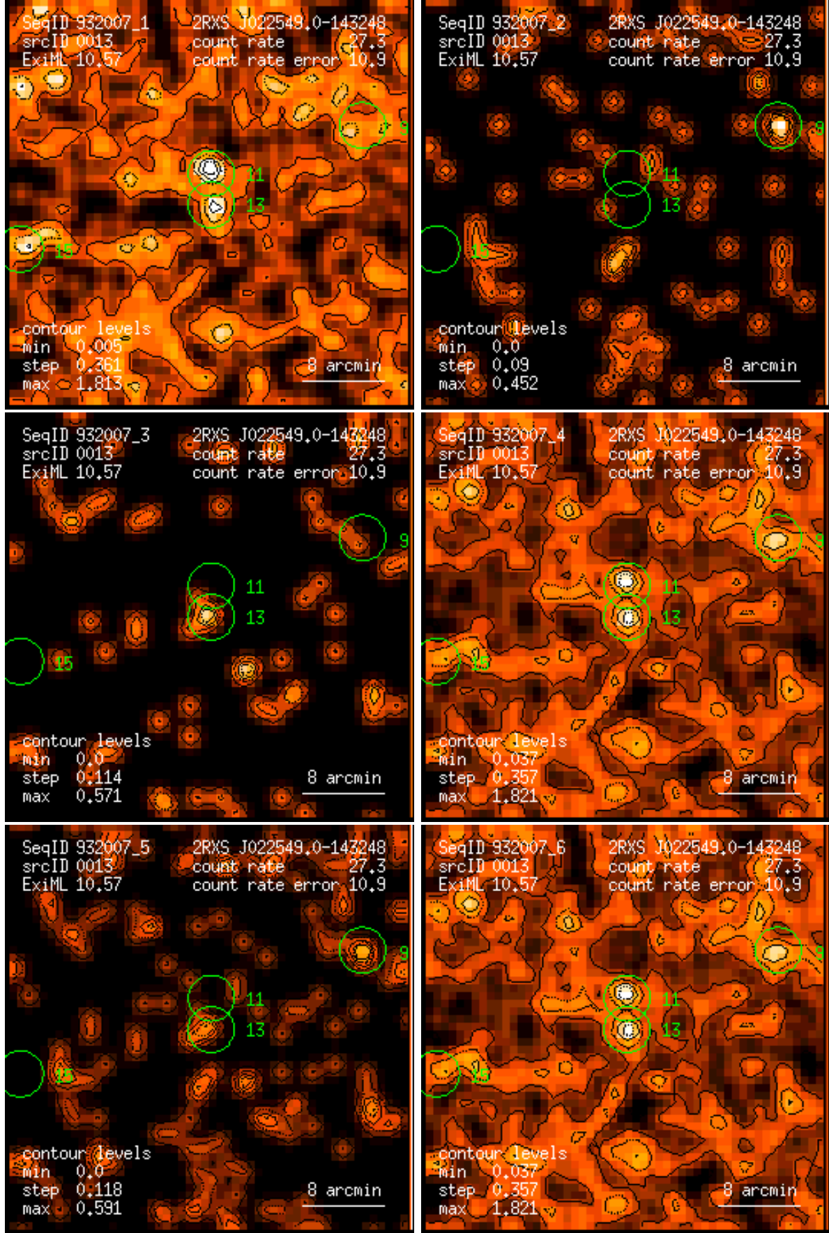
Figure 13: RASS 932007: detection 0013: band rate images, Gaussian filter: (1) PSPC channels 11 – 41, (2) 52 – 90, (3) 91 – 201, (4) 11 – 235, (5) 52 – 201, (6) 11 – 201. Broad band rates in counts/ks. Band rate contour levels in counts/ks/arcmin 2 .
