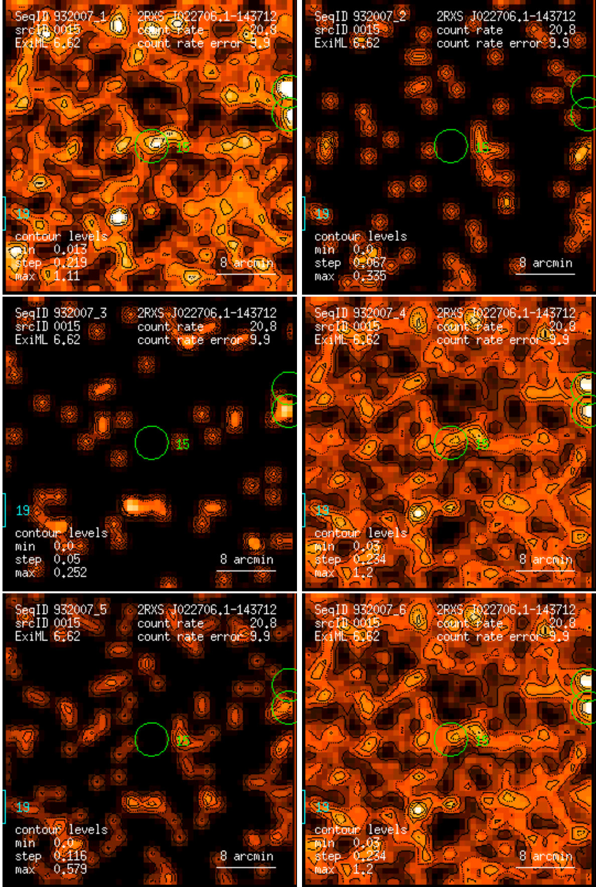
Figure 15: RASS 932007: detection 0015: band rate images, Gaussian filter: (1) PSPC channels 11 – 41, (2) 52 – 90, (3) 91 – 201, (4) 11 – 235, (5) 52 – 201, (6) 11 – 201. Broad band rates in counts/ks. Band rate contour levels in counts/ks/arcmin 2 .
