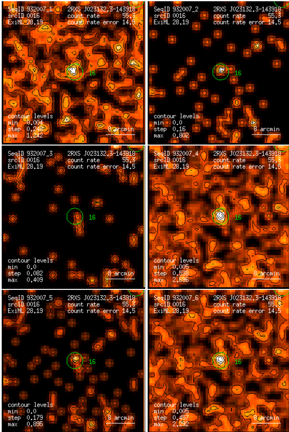
Figure 16: RASS 932007: detection 0016: band rate images, Gaussian filter: (1) PSPC channels 11 – 41, (2) 52 – 90, (3) 91 – 201, (4) 11 – 235, (5) 52 – 201, (6) 11 – 201. Broad band rates in counts/ks. Band rate contour levels in counts/ks/arcmin 2 .
