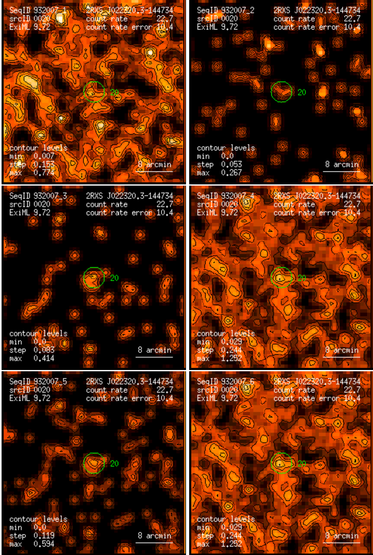
Figure 20: RASS 932007: detection 0020: band rate images, Gaussian filter: (1) PSPC channels 11 – 41, (2) 52 – 90, (3) 91 – 201, (4) 11 – 235, (5) 52 – 201, (6) 11 – 201. Broad band rates in counts/ks. Band rate contour levels in counts/ks/arcmin 2 .
