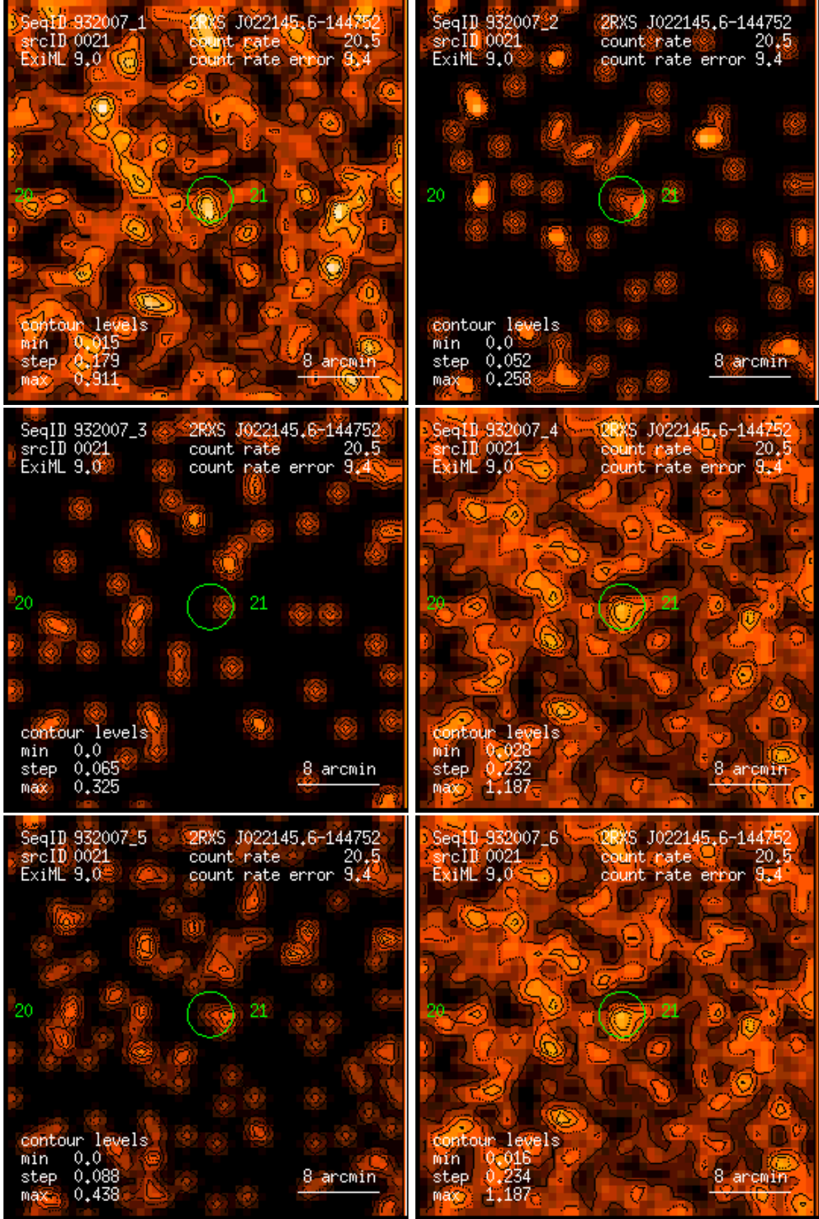
Figure 21: RASS 932007: detection 0021: band rate images, Gaussian filter: (1) PSPC channels 11 – 41, (2) 52 – 90, (3) 91 – 201, (4) 11 – 235, (5) 52 – 201, (6) 11 – 201. Broad band rates in counts/ks. Band rate contour levels in counts/ks/arcmin 2 .
