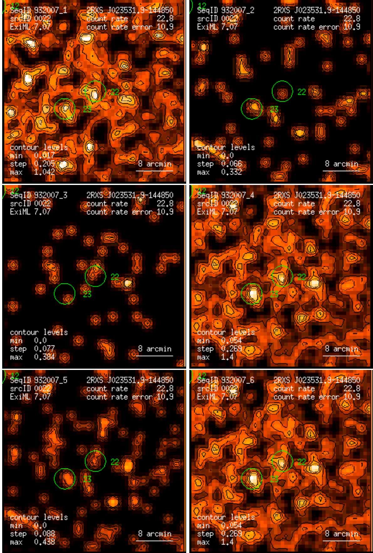
Figure 22: RASS 932007: detection 0022: band rate images, Gaussian filter: (1) PSPC channels 11 – 41, (2) 52 – 90, (3) 91 – 201, (4) 11 – 235, (5) 52 – 201, (6) 11 – 201. Broad band rates in counts/ks. Band rate contour levels in counts/ks/arcmin 2 .
