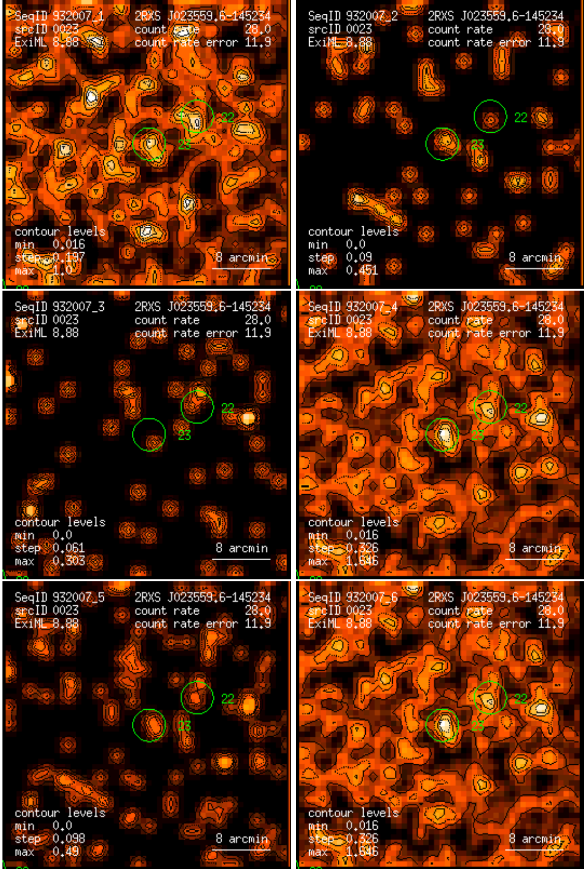
Figure 23: RASS 932007: detection 0023: band rate images, Gaussian filter: (1) PSPC channels 11 – 41, (2) 52 – 90, (3) 91 – 201, (4) 11 – 235, (5) 52 – 201, (6) 11 – 201. Broad band rates in counts/ks. Band rate contour levels in counts/ks/arcmin 2 .
