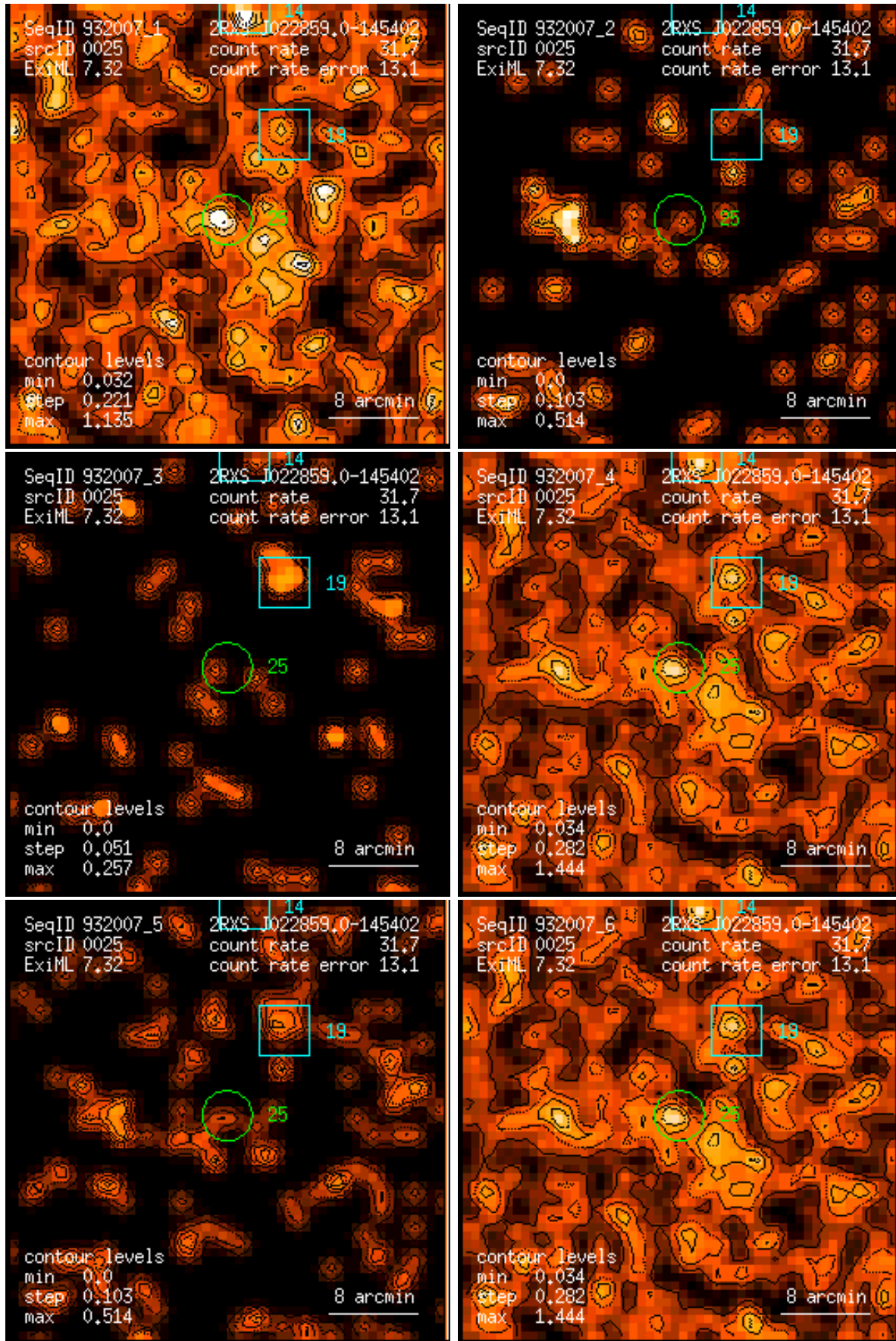
Figure 25: RASS 932007: detection 0025: band rate images, Gaussian filter: (1) PSPC channels 11 – 41, (2) 52 – 90, (3) 91 – 201, (4) 11 – 235, (5) 52 – 201, (6) 11 – 201. Broad band rates in counts/ks. Band rate contour levels in counts/ks/arcmin 2 .
