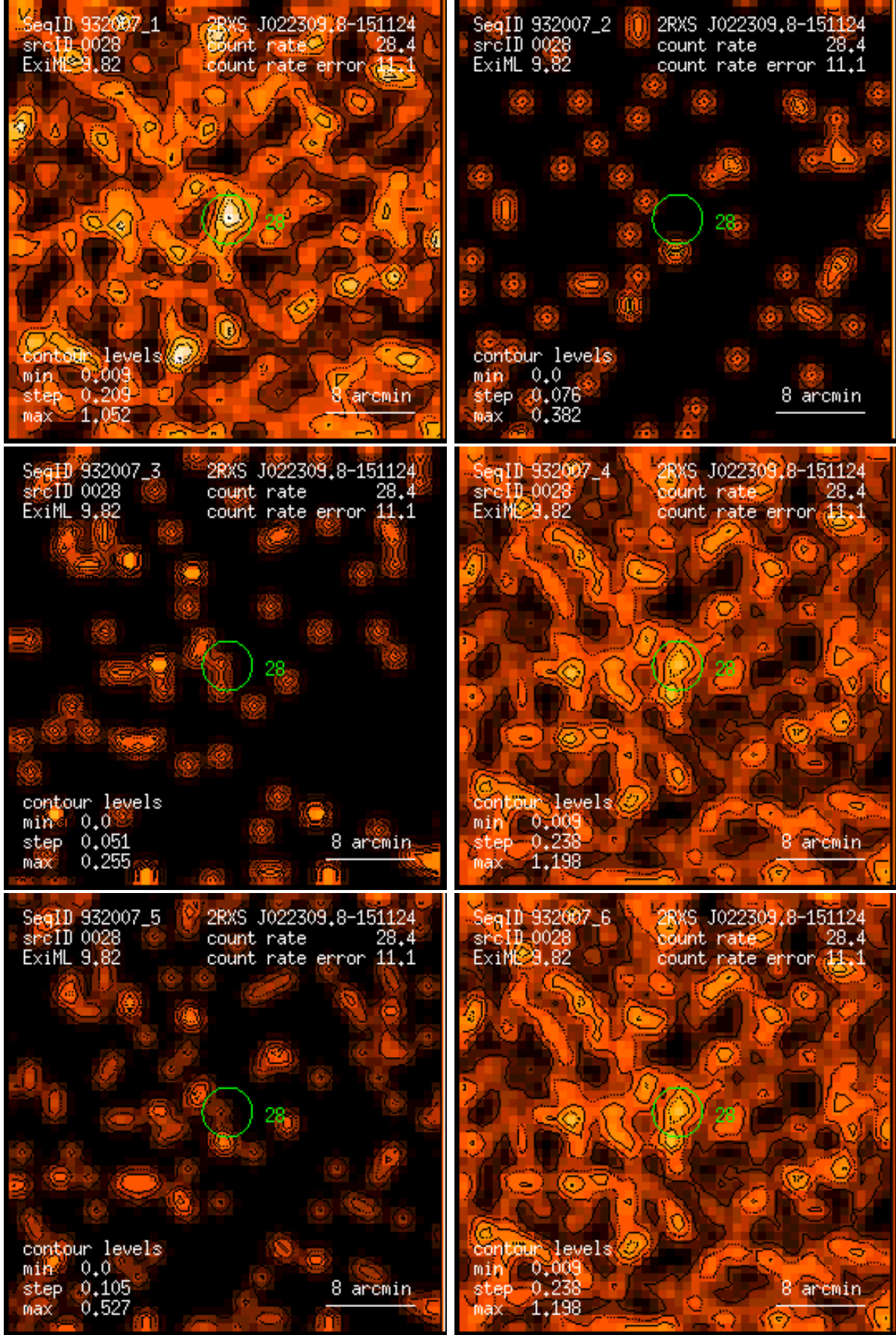
Figure 28: RASS 932007: detection 0028: band rate images, Gaussian filter: (1) PSPC channels 11 – 41, (2) 52 – 90, (3) 91 – 201, (4) 11 – 235, (5) 52 – 201, (6) 11 – 201. Broad band rates in counts/ks. Band rate contour levels in counts/ks/arcmin 2 .
