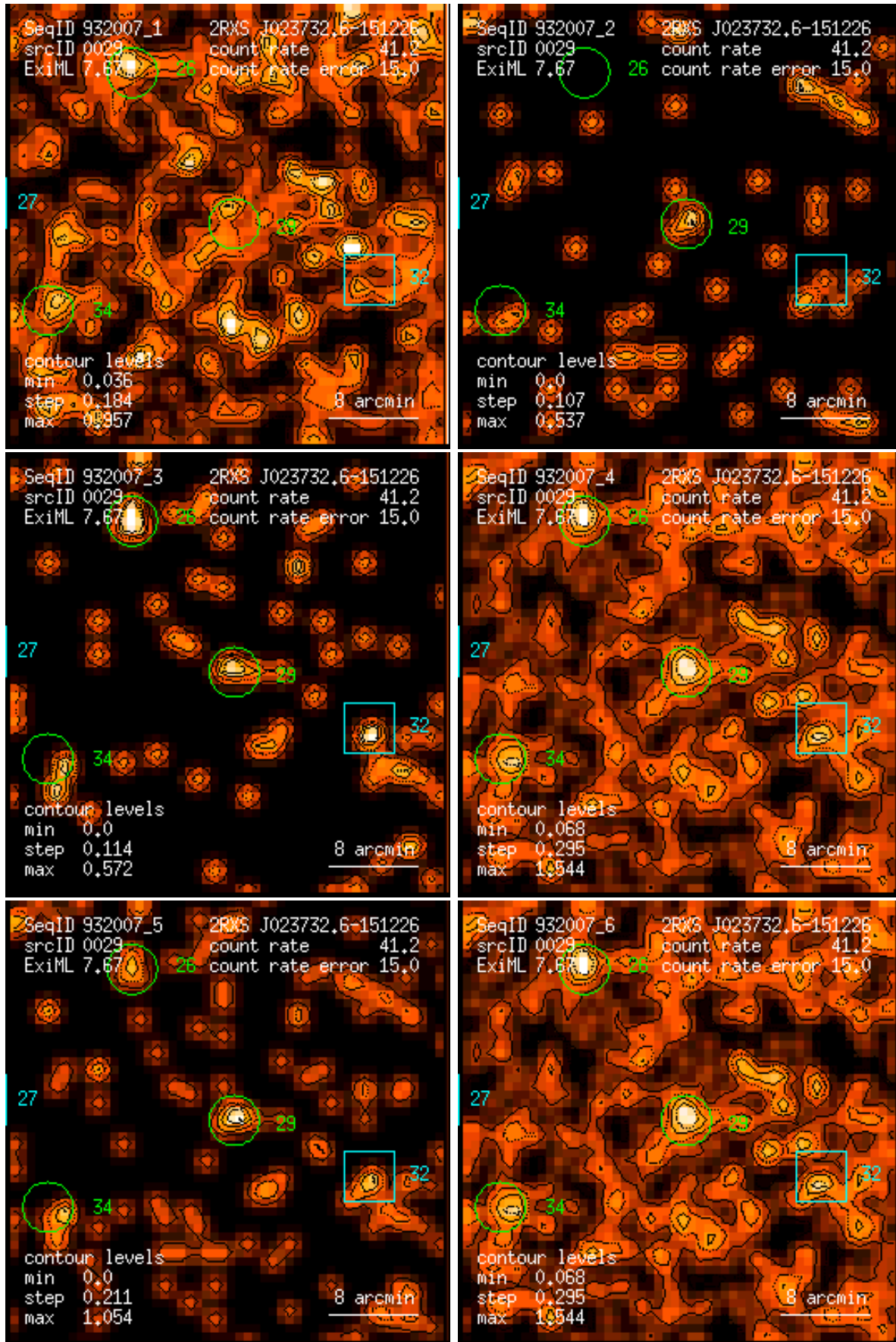
Figure 29: RASS 932007: detection 0029: band rate images, Gaussian filter: (1) PSPC channels 11 – 41, (2) 52 – 90, (3) 91 – 201, (4) 11 – 235, (5) 52 – 201, (6) 11 – 201. Broad band rates in counts/ks. Band rate contour levels in counts/ks/arcmin 2 .
