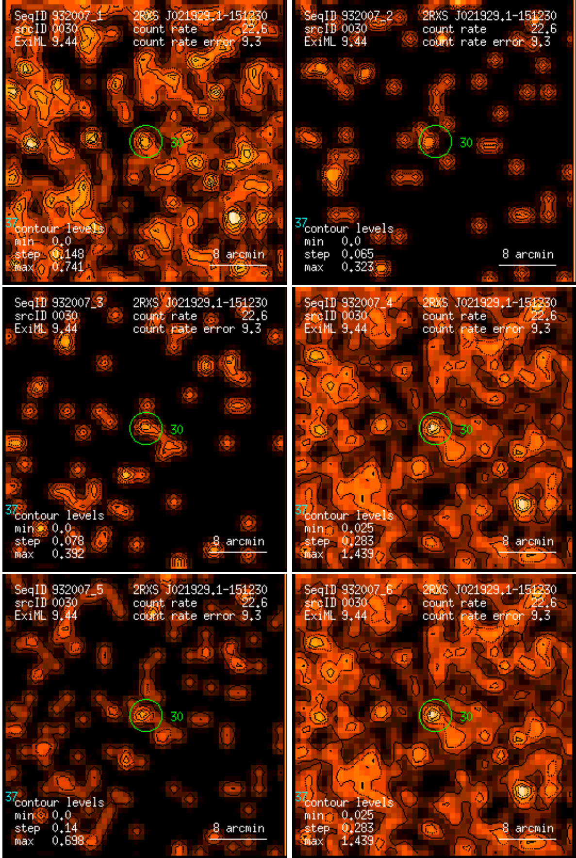
Figure 30: RASS 932007: detection 0030: band rate images, Gaussian filter: (1) PSPC channels 11 – 41, (2) 52 – 90, (3) 91 – 201, (4) 11 – 235, (5) 52 – 201, (6) 11 – 201. Broad band rates in counts/ks. Band rate contour levels in counts/ks/arcmin 2 .
