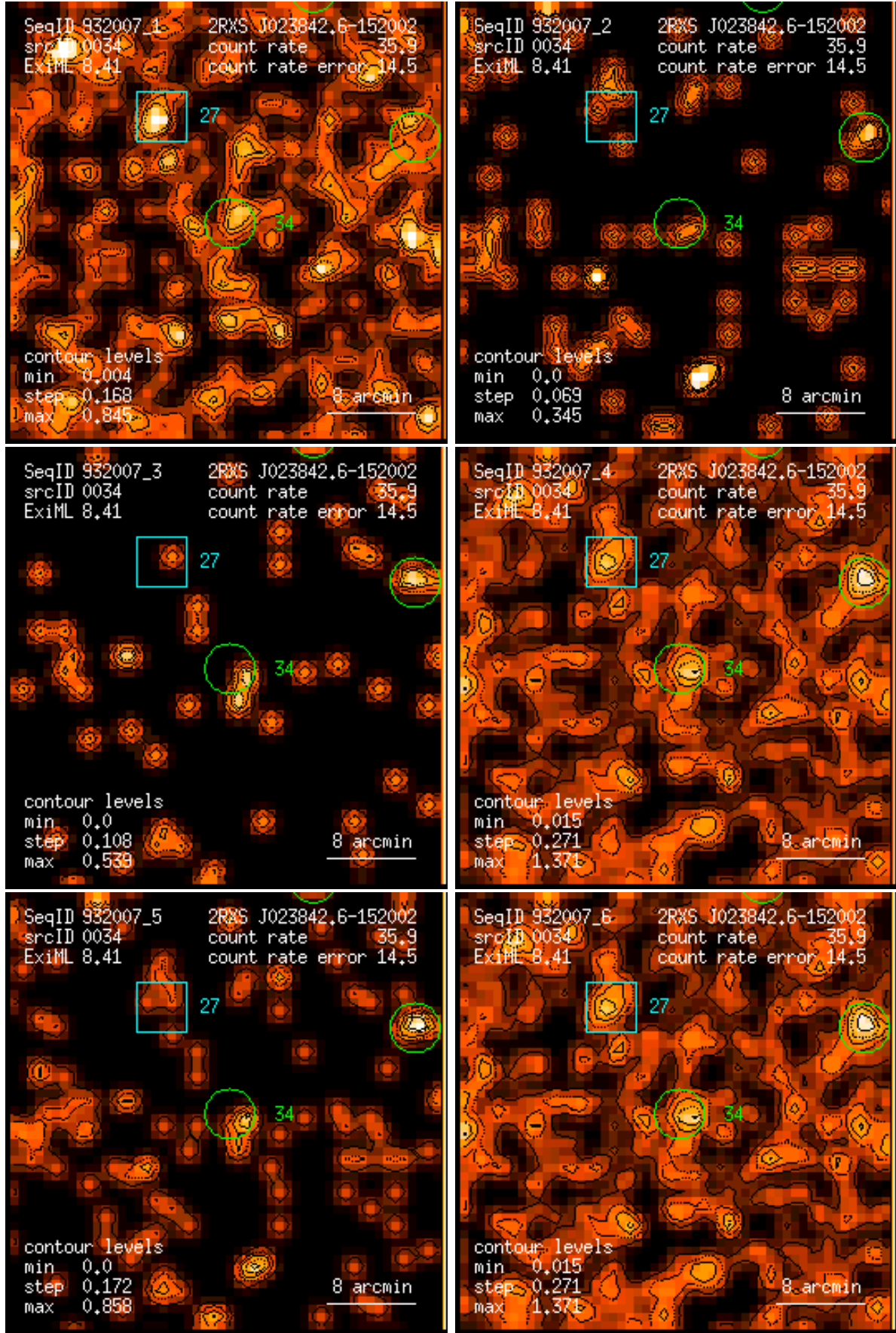
Figure 34: RASS 932007: detection 0034: band rate images, Gaussian filter: (1) PSPC channels 11 – 41, (2) 52 – 90, (3) 91 – 201, (4) 11 – 235, (5) 52 – 201, (6) 11 – 201. Broad band rates in counts/ks. Band rate contour levels in counts/ks/arcmin 2 .
