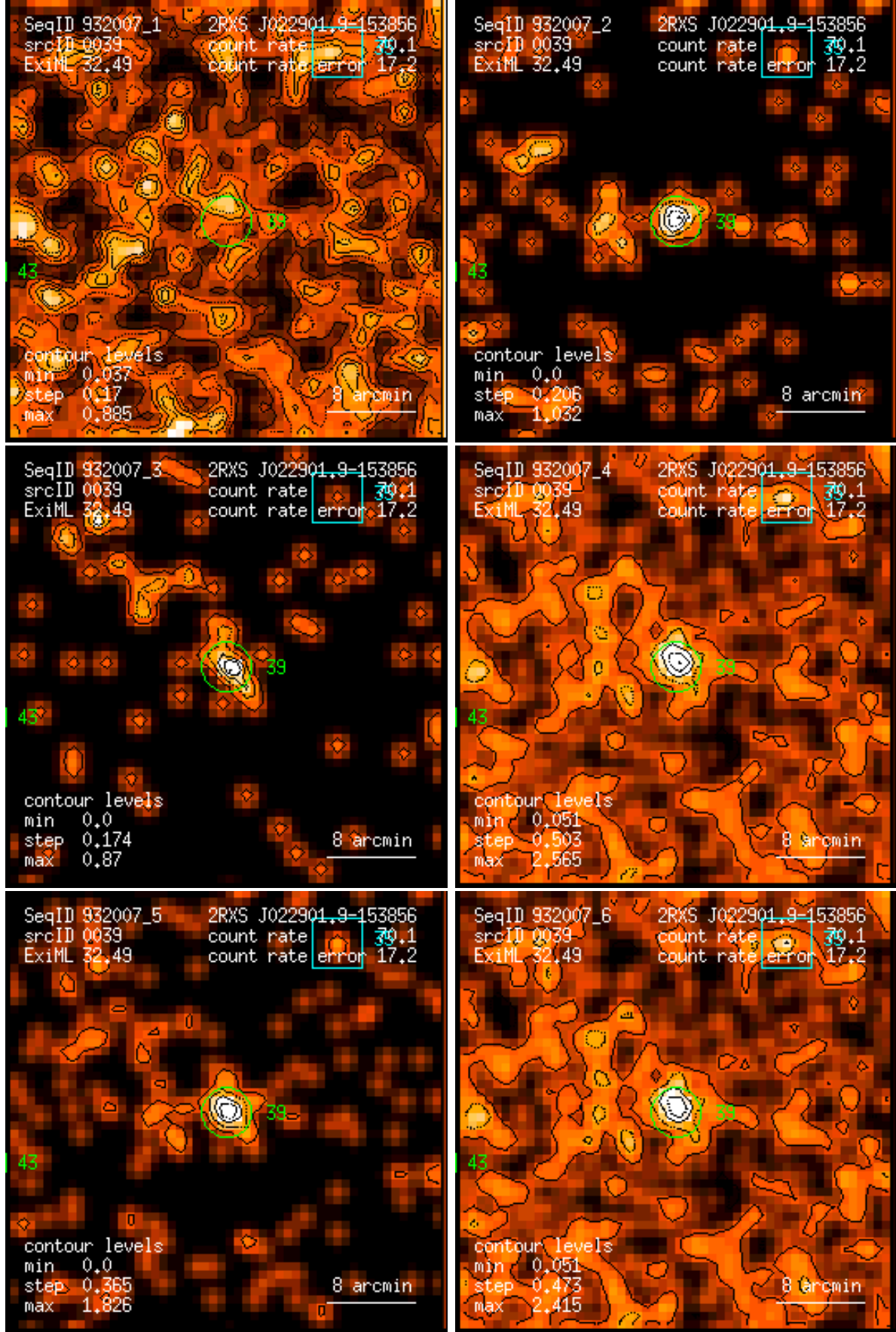
Figure 39: RASS 932007: detection 0039: band rate images, Gaussian filter: (1) PSPC channels 11 – 41, (2) 52 – 90, (3) 91 – 201, (4) 11 – 235, (5) 52 – 201, (6) 11 – 201. Broad band rates in counts/ks. Band rate contour levels in counts/ks/arcmin 2 .
