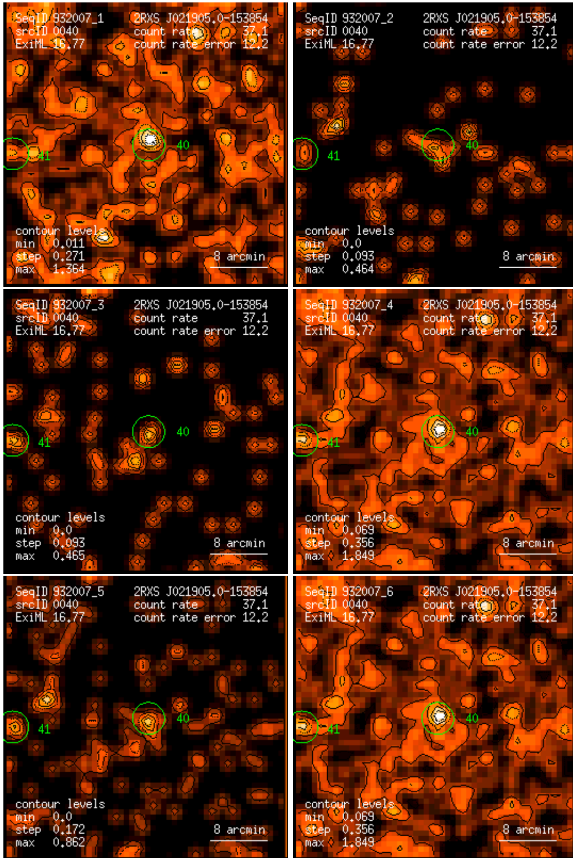
Figure 40: RASS 932007: detection 0040: band rate images, Gaussian filter: (1) PSPC channels 11 – 41, (2) 52 – 90, (3) 91 – 201, (4) 11 – 235, (5) 52 – 201, (6) 11 – 201. Broad band rates in counts/ks. Band rate contour levels in counts/ks/arcmin 2 .
