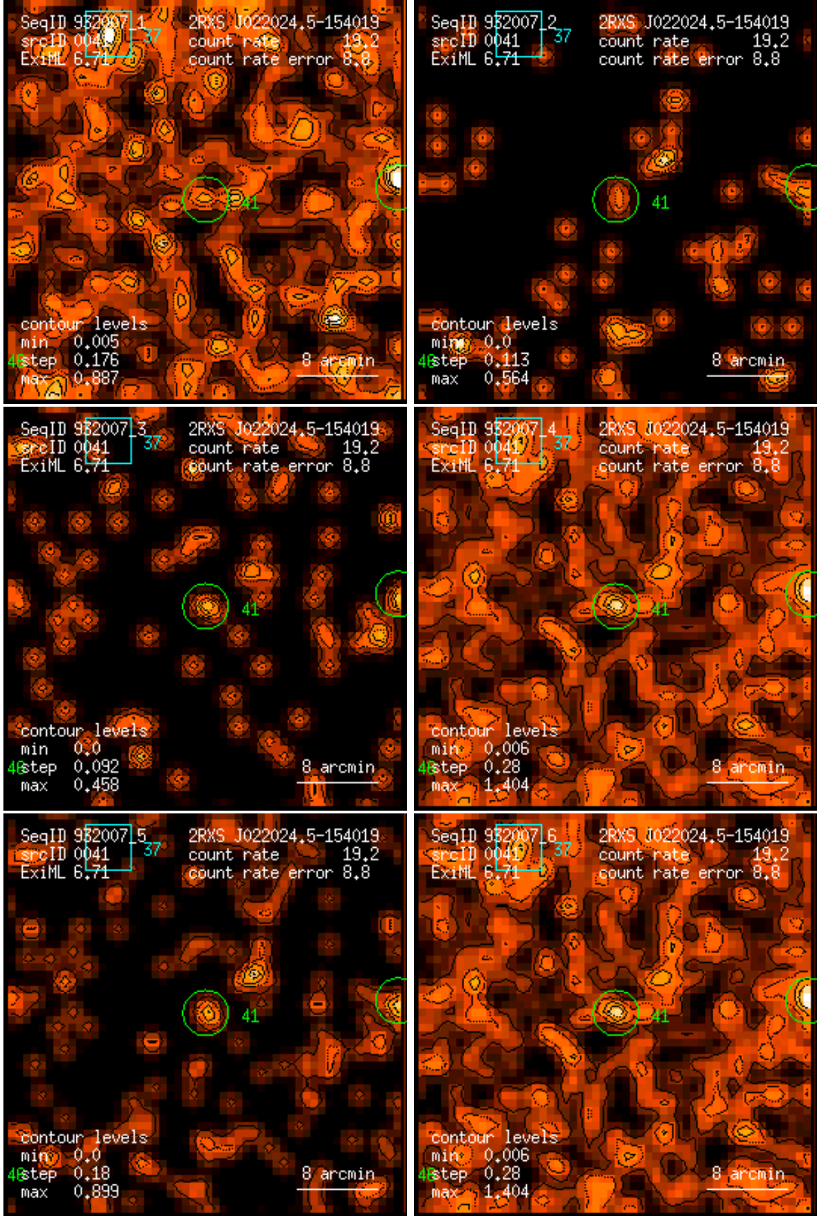
Figure 41: RASS 932007: detection 0041: band rate images, Gaussian filter: (1) PSPC channels 11 – 41, (2) 52 – 90, (3) 91 – 201, (4) 11 – 235, (5) 52 – 201, (6) 11 – 201. Broad band rates in counts/ks. Band rate contour levels in counts/ks/arcmin 2 .
