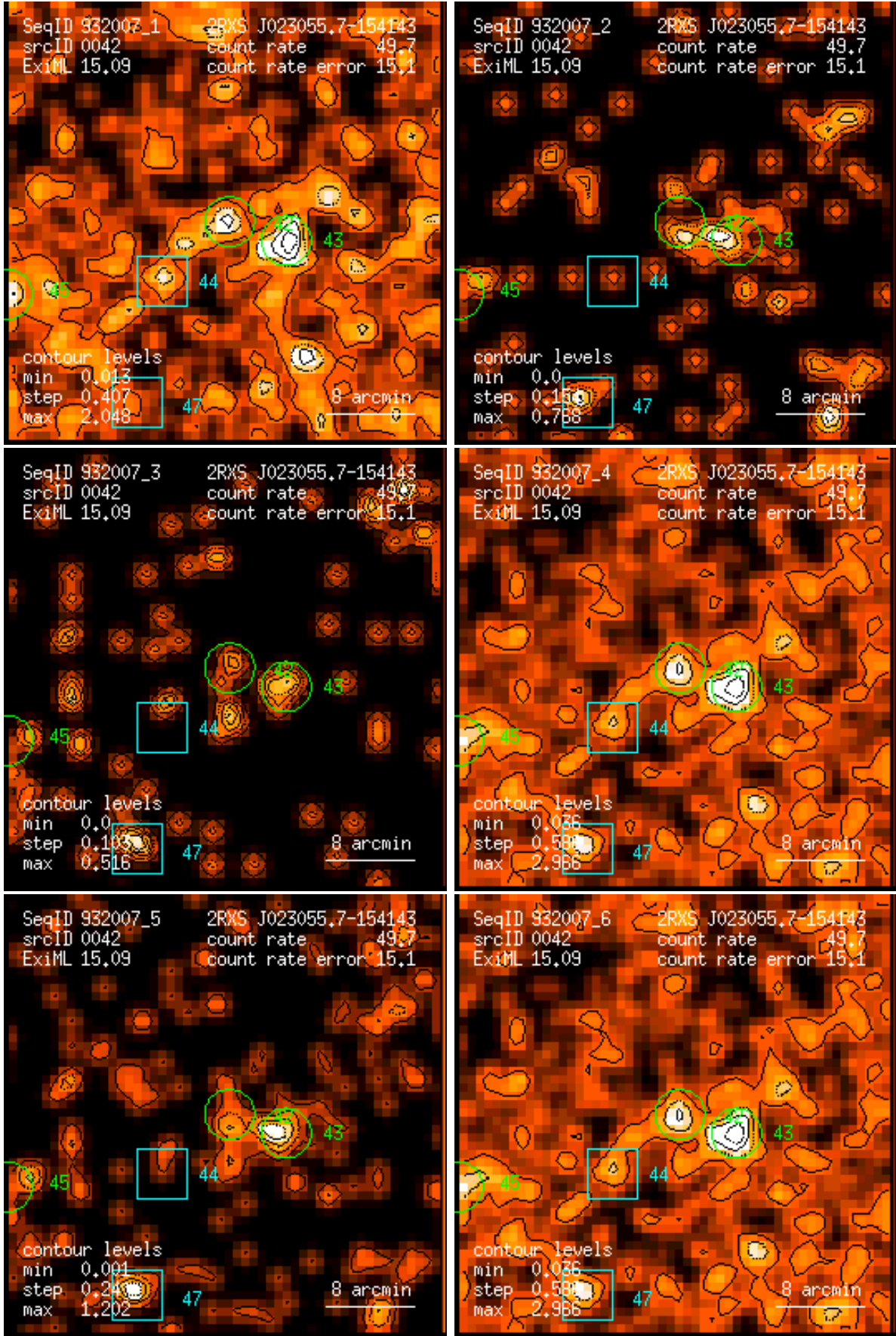
Figure 42: RASS 932007: detection 0042: band rate images, Gaussian filter: (1) PSPC channels 11 – 41, (2) 52 – 90, (3) 91 – 201, (4) 11 – 235, (5) 52 – 201, (6) 11 – 201. Broad band rates in counts/ks. Band rate contour levels in counts/ks/arcmin 2 .
