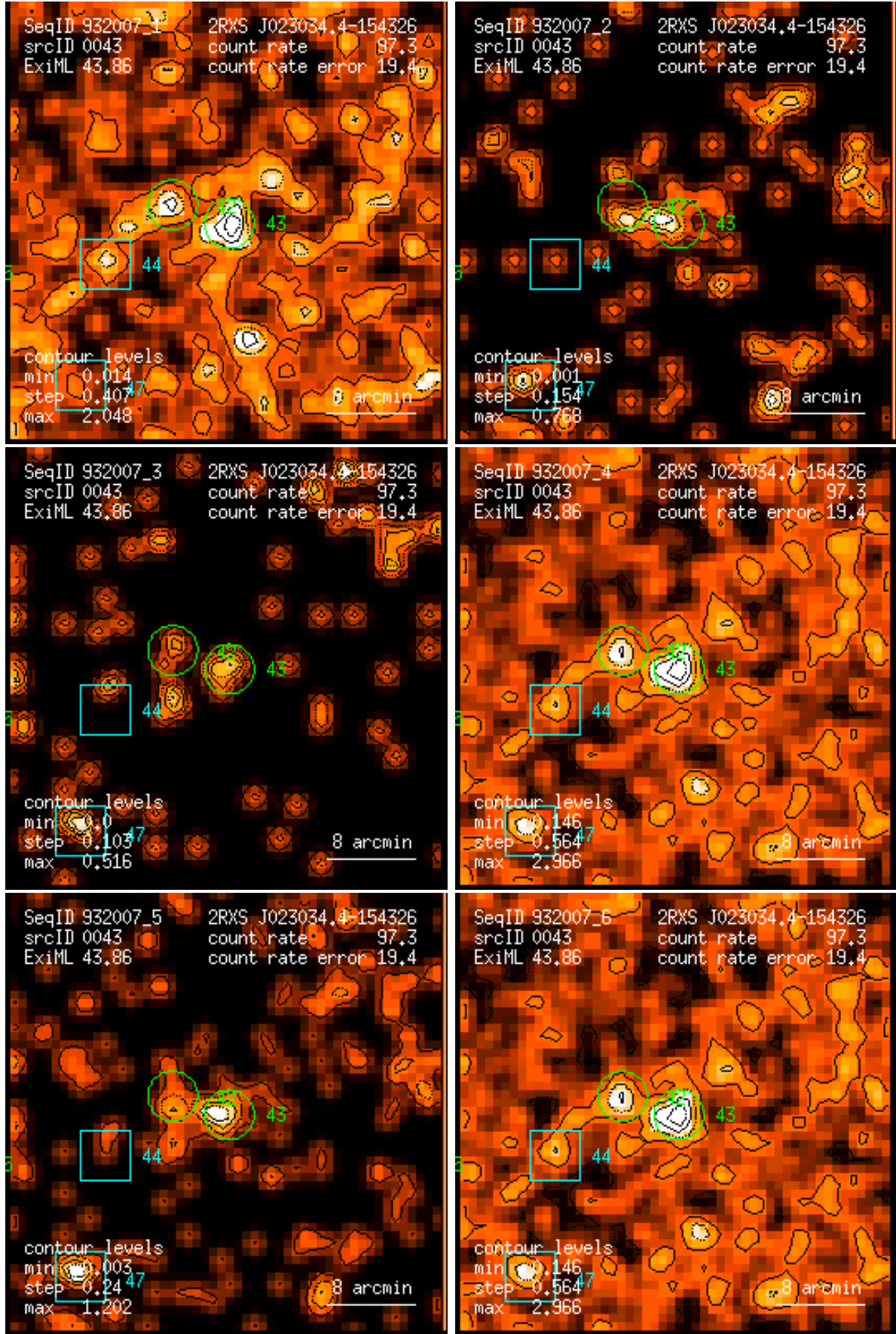
Figure 43: RASS 932007: detection 0043: band rate images, Gaussian filter: (1) PSPC channels 11 – 41, (2) 52 – 90, (3) 91 – 201, (4) 11 – 235, (5) 52 – 201, (6) 11 – 201. Broad band rates in counts/ks. Band rate contour levels in counts/ks/arcmin 2 .
