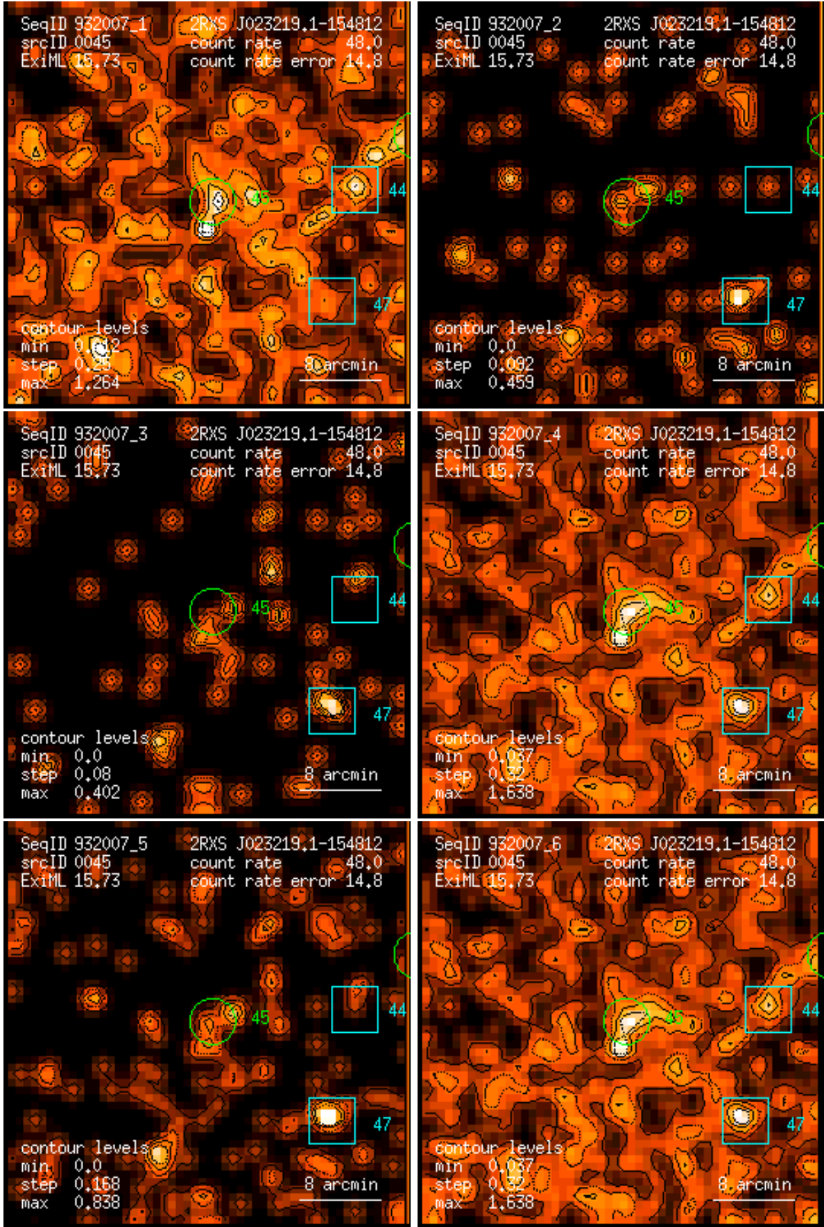
Figure 45: RASS 932007: detection 0045: band rate images, Gaussian filter: (1) PSPC channels 11 – 41, (2) 52 – 90, (3) 91 – 201, (4) 11 – 235, (5) 52 – 201, (6) 11 – 201. Broad band rates in counts/ks. Band rate contour levels in counts/ks/arcmin 2 .
