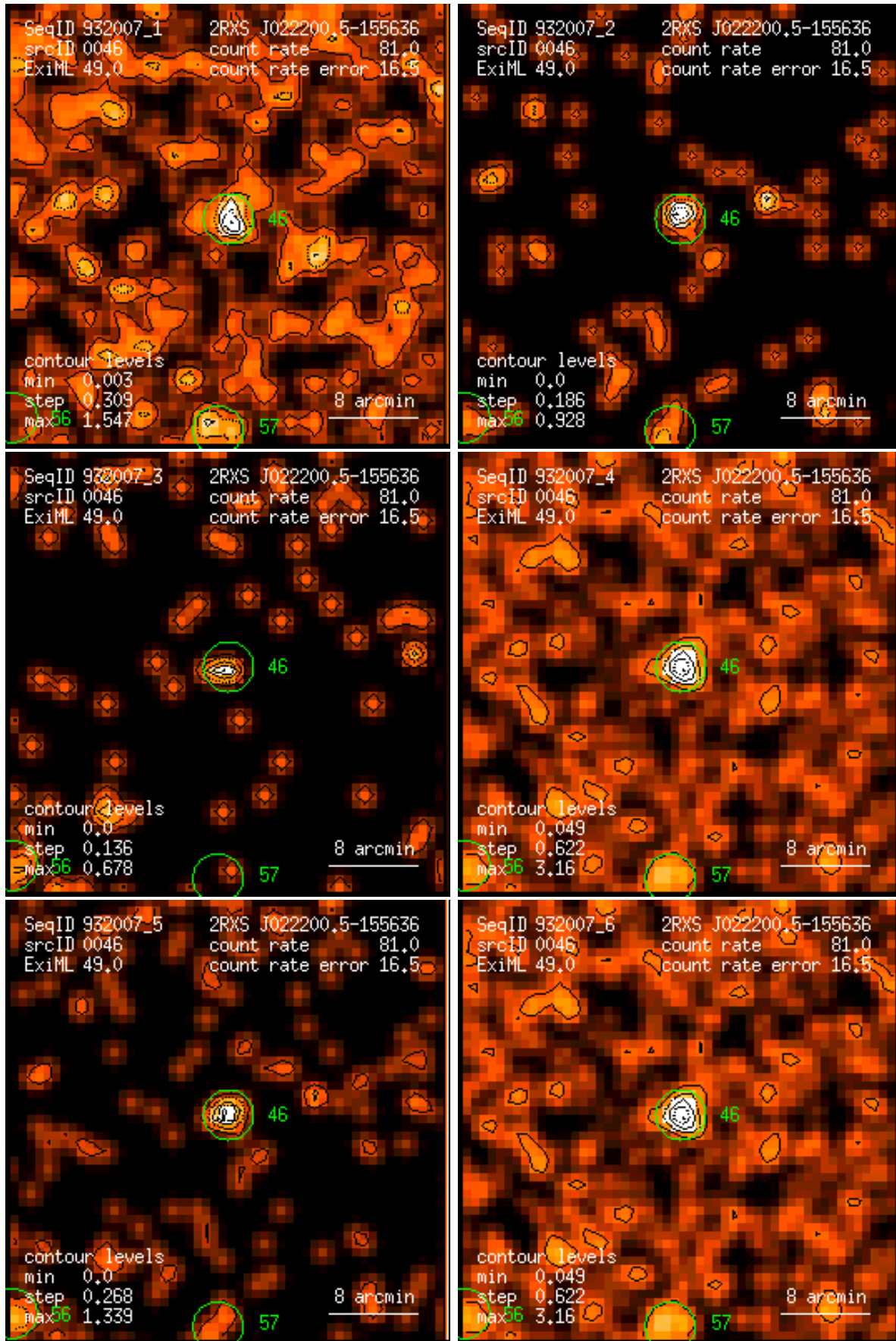
Figure 46: RASS 932007: detection 0046: band rate images, Gaussian filter: (1) PSPC channels 11 – 41, (2) 52 – 90, (3) 91 – 201, (4) 11 – 235, (5) 52 – 201, (6) 11 – 201. Broad band rates in counts/ks. Band rate contour levels in counts/ks/arcmin 2 .
