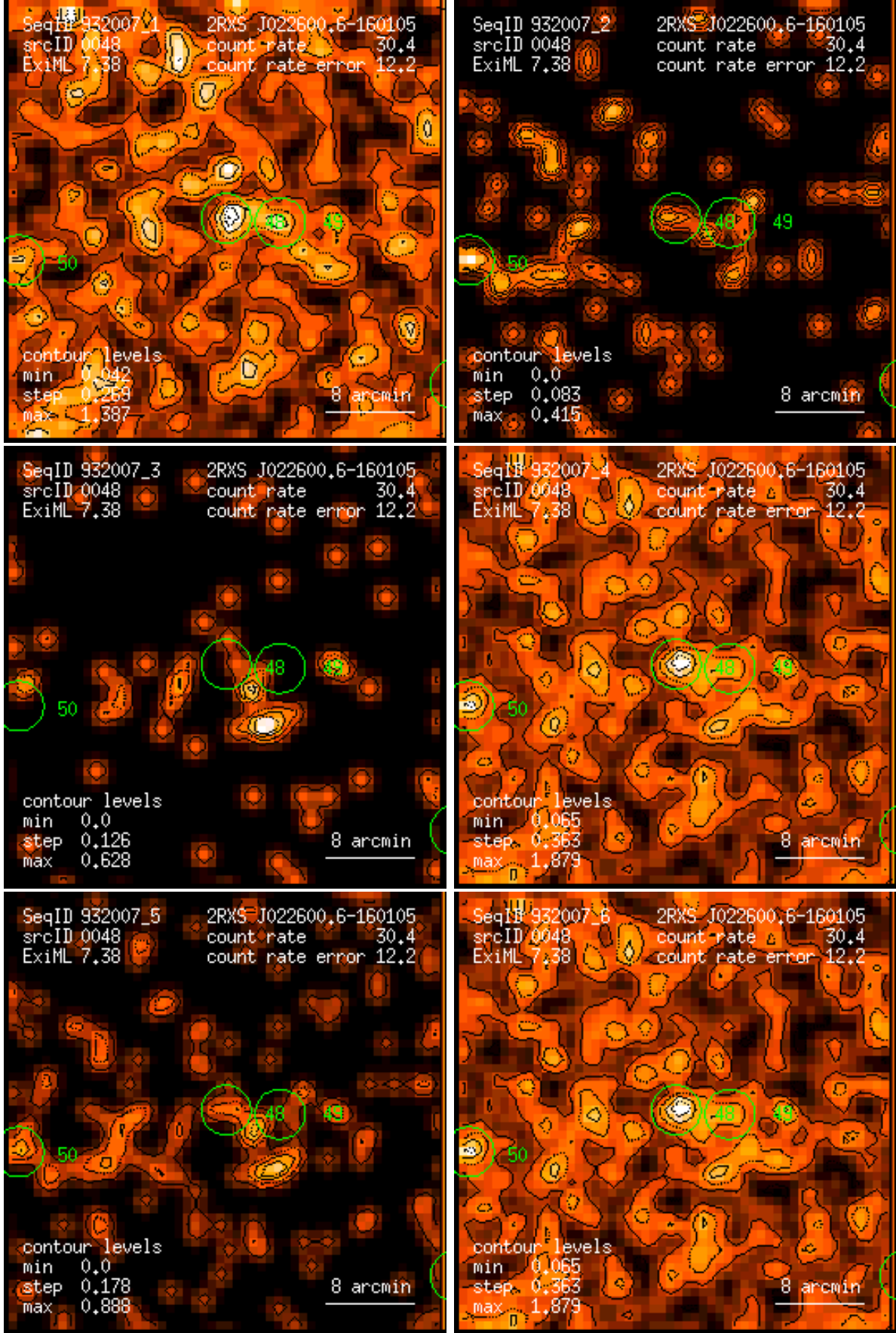
Figure 48: RASS 932007: detection 0048: band rate images, Gaussian filter: (1) PSPC channels 11 – 41, (2) 52 – 90, (3) 91 – 201, (4) 11 – 235, (5) 52 – 201, (6) 11 – 201. Broad band rates in counts/ks. Band rate contour levels in counts/ks/arcmin 2 .
