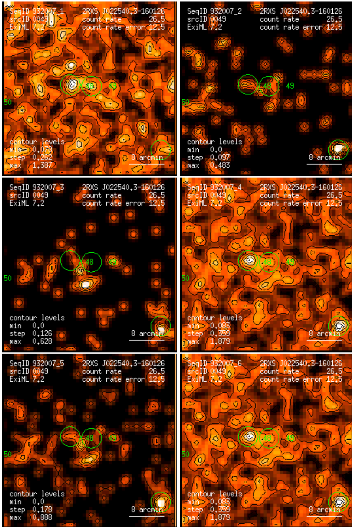
Figure 49: RASS 932007: detection 0049: band rate images, Gaussian filter: (1) PSPC channels 11 – 41, (2) 52 – 90, (3) 91 – 201, (4) 11 – 235, (5) 52 – 201, (6) 11 – 201. Broad band rates in counts/ks. Band rate contour levels in counts/ks/arcmin 2 .
