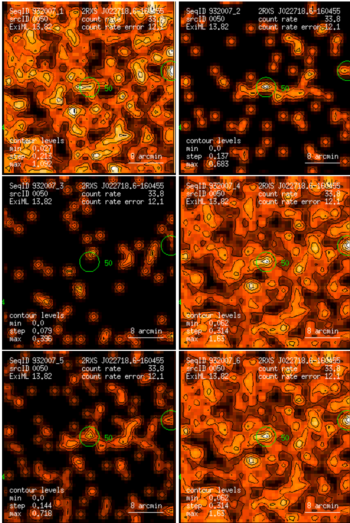
Figure 50: RASS 932007: detection 0050: band rate images, Gaussian filter: (1) PSPC channels 11 – 41, (2) 52 – 90, (3) 91 – 201, (4) 11 – 235, (5) 52 – 201, (6) 11 – 201. Broad band rates in counts/ks. Band rate contour levels in counts/ks/arcmin 2 .
