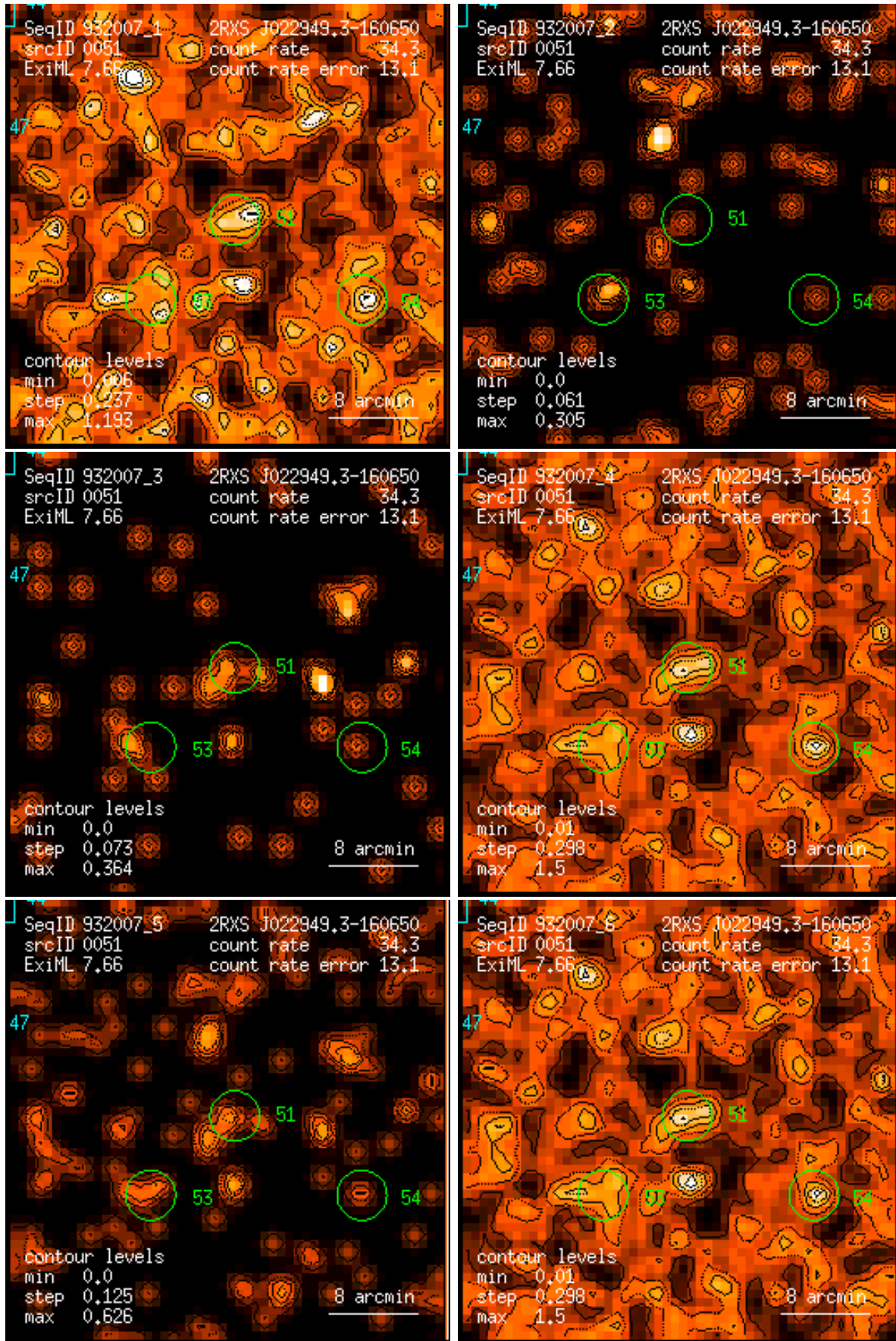
Figure 51: RASS 932007: detection 0051: band rate images, Gaussian filter: (1) PSPC channels 11 – 41, (2) 52 – 90, (3) 91 – 201, (4) 11 – 235, (5) 52 – 201, (6) 11 – 201. Broad band rates in counts/ks. Band rate contour levels in counts/ks/arcmin 2 .
