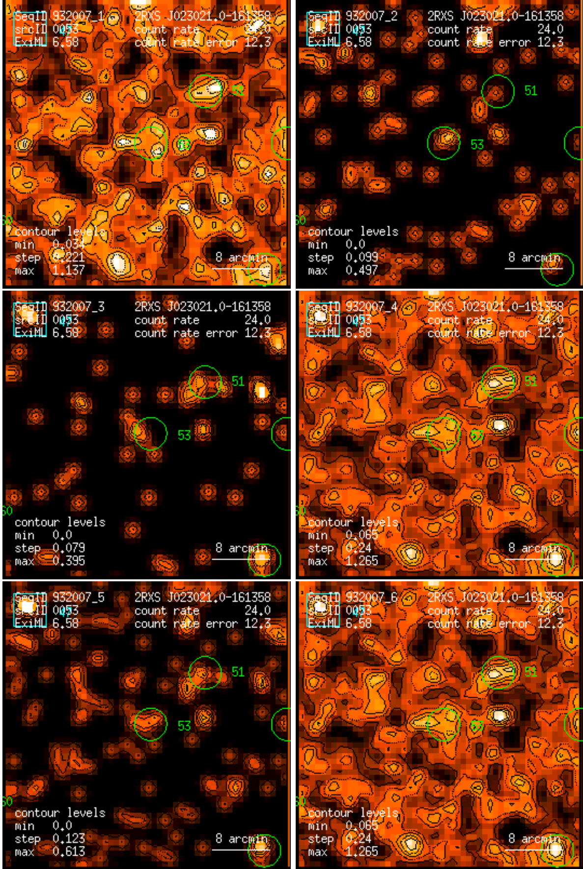
Figure 53: RASS 932007: detection 0053: band rate images, Gaussian filter: (1) PSPC channels 11 – 41, (2) 52 – 90, (3) 91 – 201, (4) 11 – 235, (5) 52 – 201, (6) 11 – 201. Broad band rates in counts/ks. Band rate contour levels in counts/ks/arcmin 2 .
