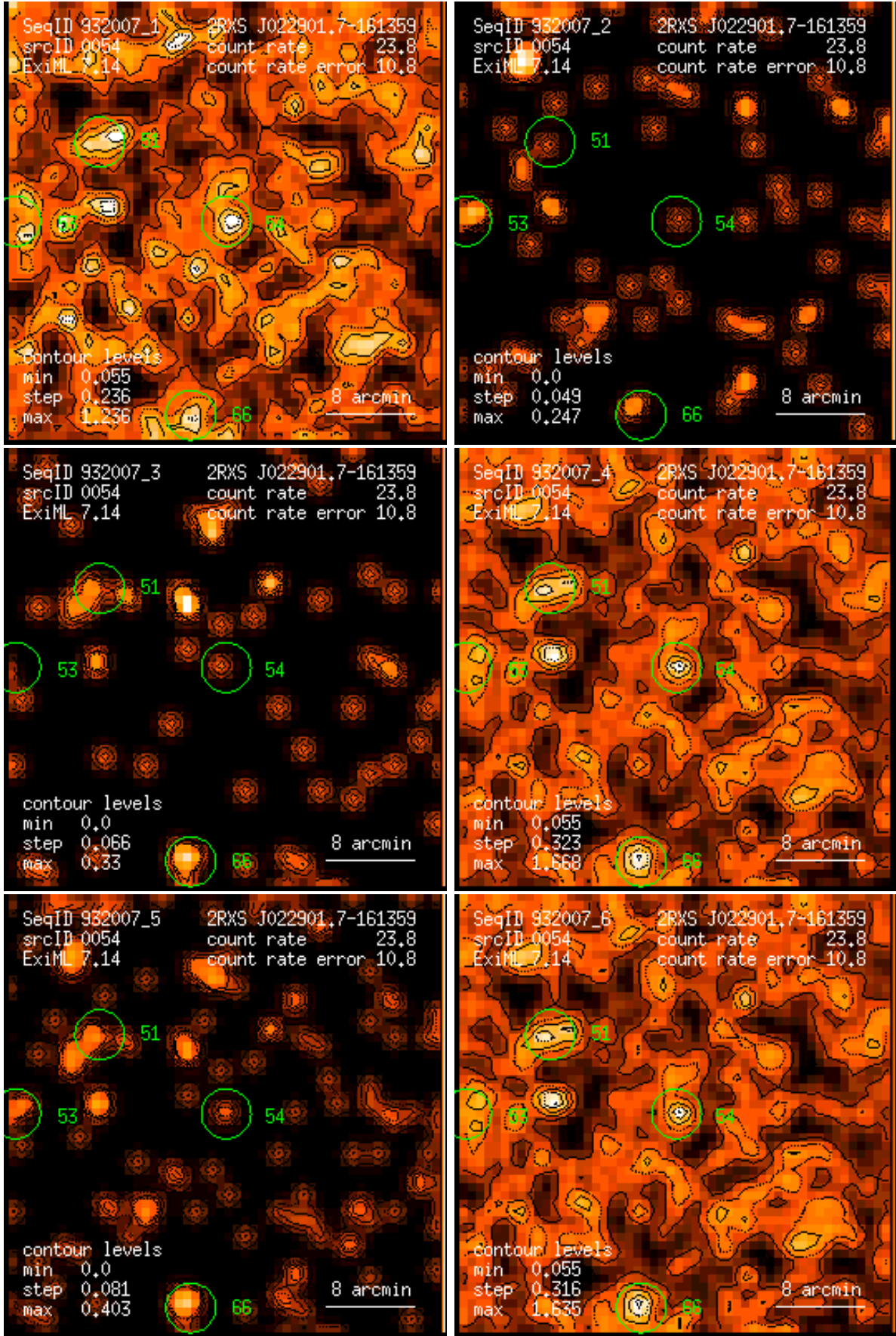
Figure 54: RASS 932007: detection 0054: band rate images, Gaussian filter: (1) PSPC channels 11 – 41, (2) 52 – 90, (3) 91 – 201, (4) 11 – 235, (5) 52 – 201, (6) 11 – 201. Broad band rates in counts/ks. Band rate contour levels in counts/ks/arcmin 2 .
