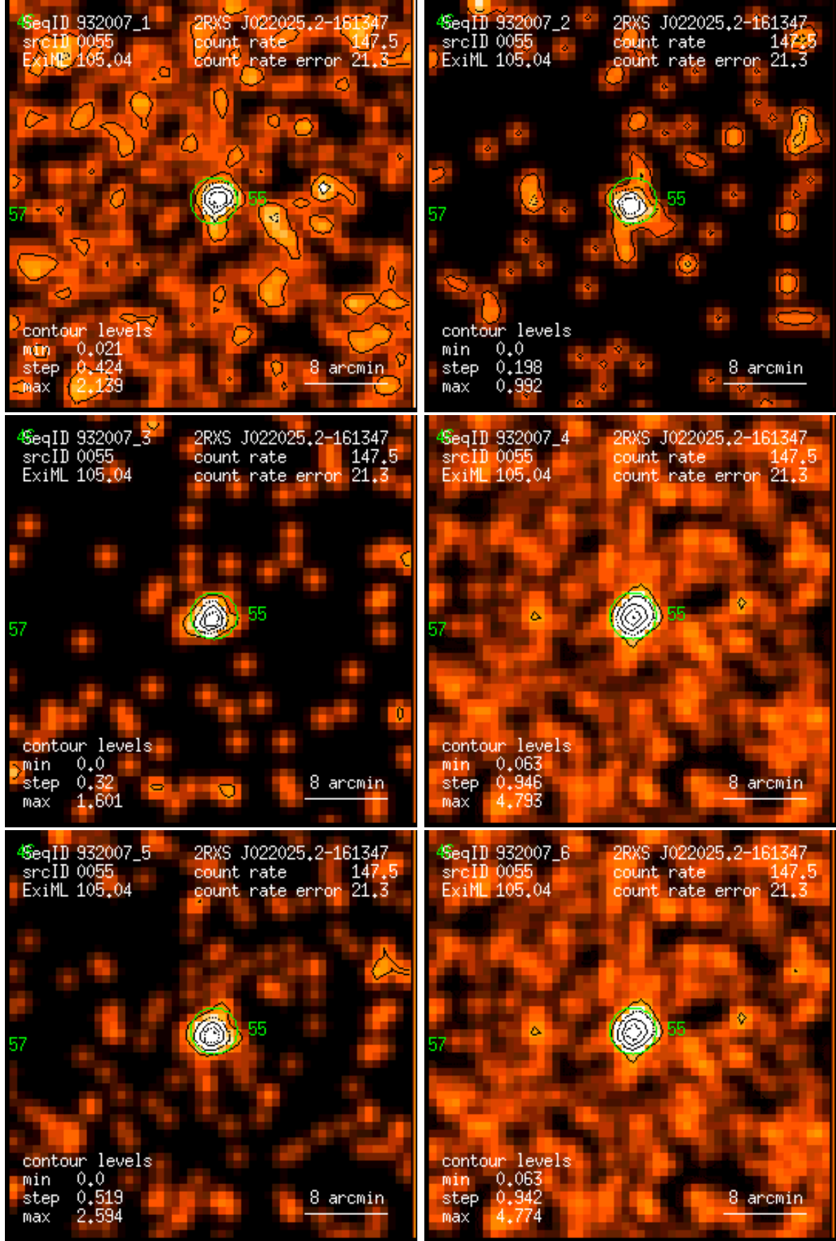
Figure 55: RASS 932007: detection 0055: band rate images, Gaussian filter: (1) PSPC channels 11 – 41, (2) 52 – 90, (3) 91 – 201, (4) 11 – 235, (5) 52 – 201, (6) 11 – 201. Broad band rates in counts/ks. Band rate contour levels in counts/ks/arcmin 2 .
