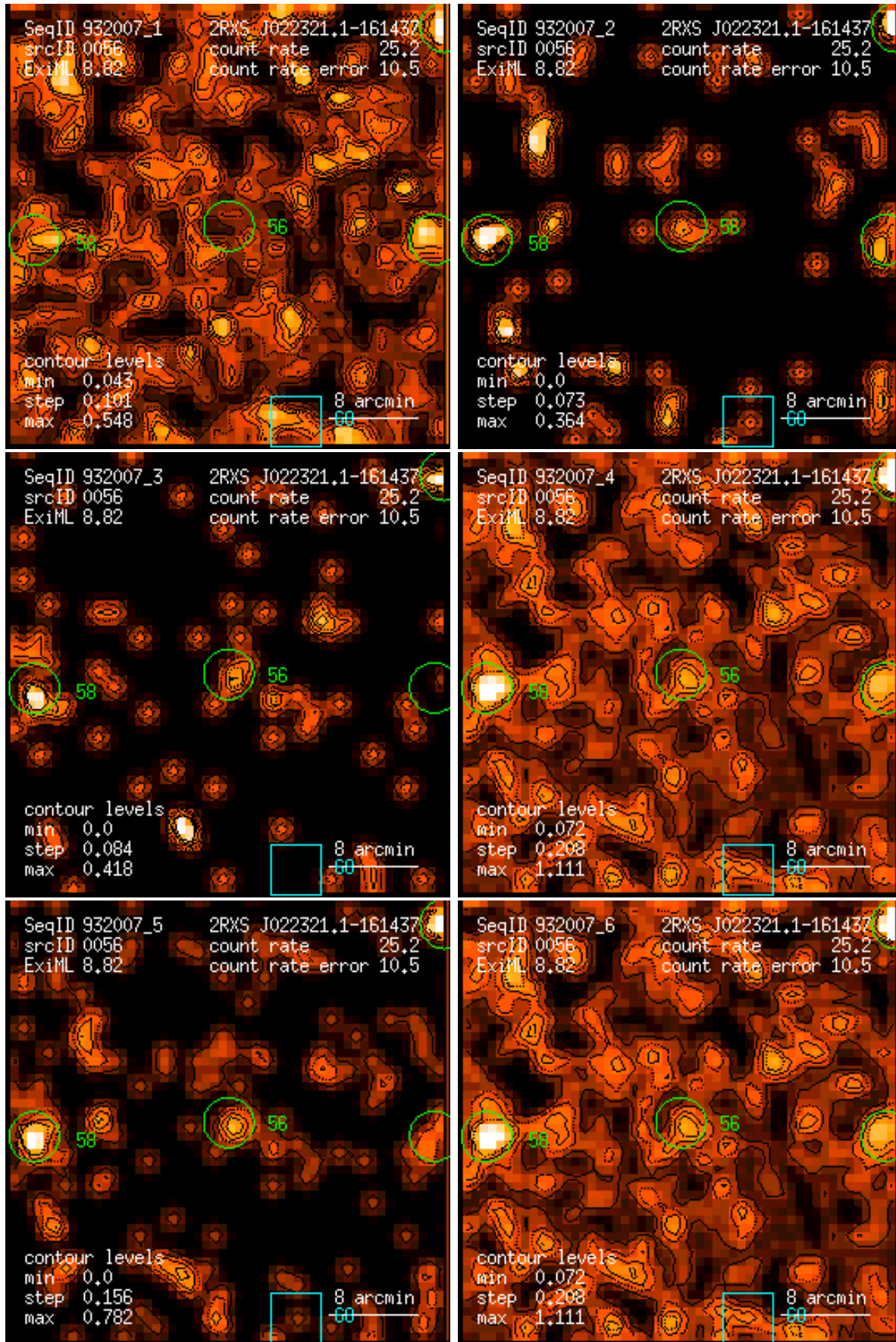
Figure 56: RASS 932007: detection 0056: band rate images, Gaussian filter: (1) PSPC channels 11 – 41, (2) 52 – 90, (3) 91 – 201, (4) 11 – 235, (5) 52 – 201, (6) 11 – 201. Broad band rates in counts/ks. Band rate contour levels in counts/ks/arcmin 2 .
