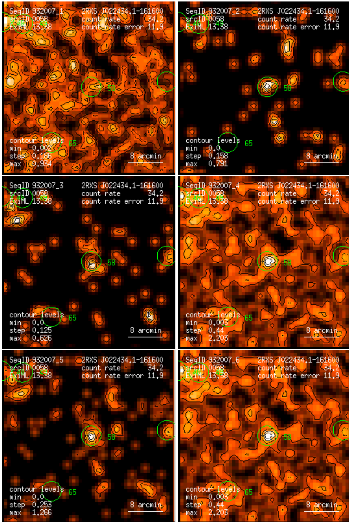
Figure 58: RASS 932007: detection 0058: band rate images, Gaussian filter: (1) PSPC channels 11 – 41, (2) 52 – 90, (3) 91 – 201, (4) 11 – 235, (5) 52 – 201, (6) 11 – 201. Broad band rates in counts/ks. Band rate contour levels in counts/ks/arcmin 2 .
