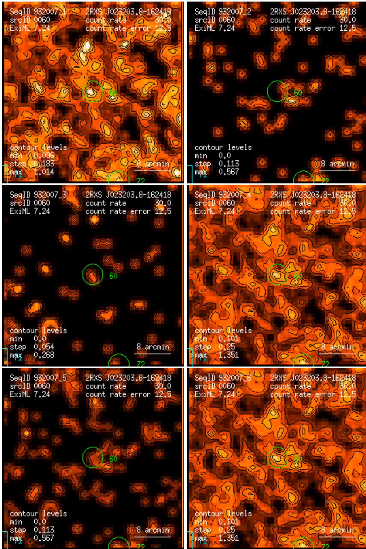
Figure 60: RASS 932007: detection 0060: band rate images, Gaussian filter: (1) PSPC channels 11 – 41, (2) 52 – 90, (3) 91 – 201, (4) 11 – 235, (5) 52 – 201, (6) 11 – 201. Broad band rates in counts/ks. Band rate contour levels in counts/ks/arcmin 2 .
