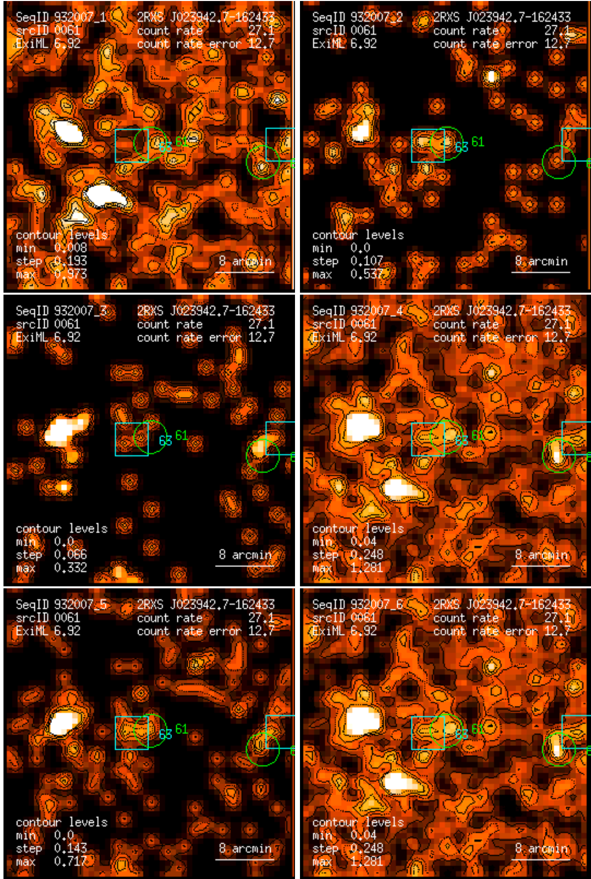
Figure 61: RASS 932007: detection 0061: band rate images, Gaussian filter: (1) PSPC channels 11 – 41, (2) 52 – 90, (3) 91 – 201, (4) 11 – 235, (5) 52 – 201, (6) 11 – 201. Broad band rates in counts/ks. Band rate contour levels in counts/ks/arcmin 2 .
