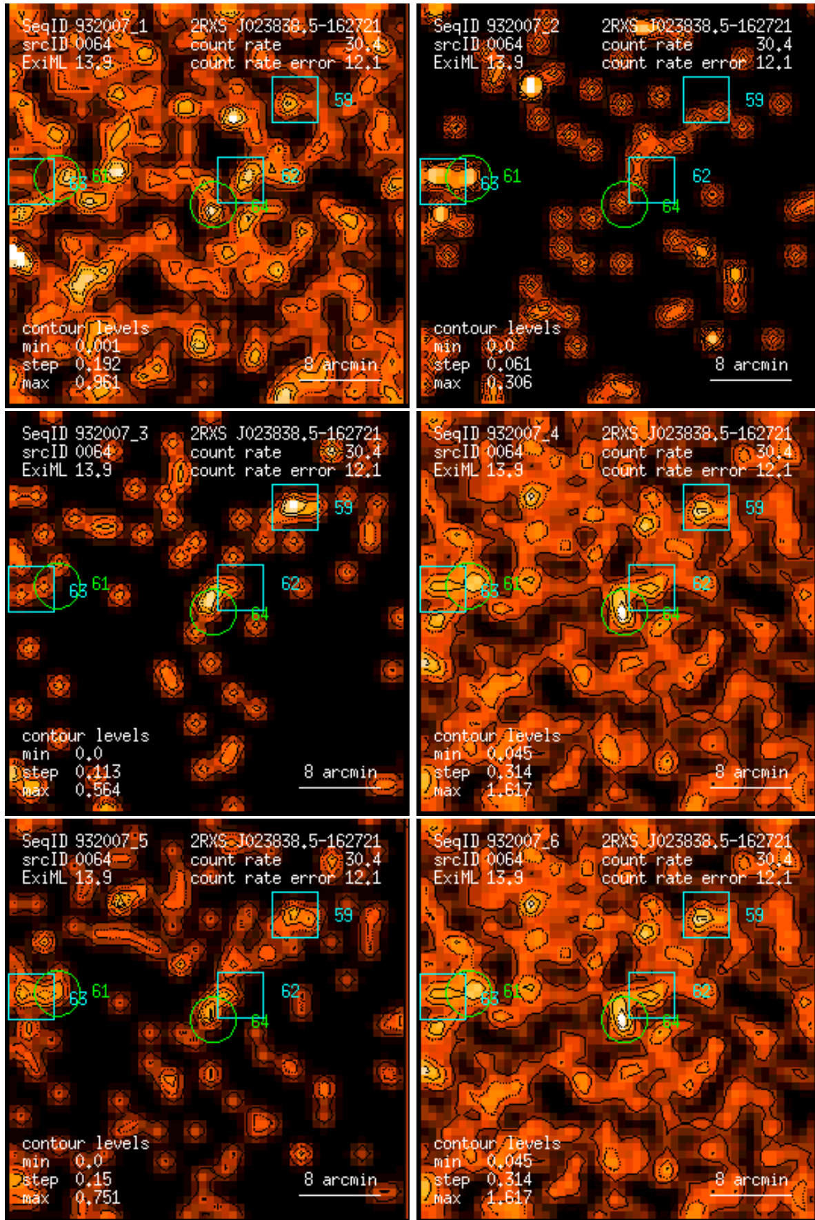
Figure 64: RASS 932007: detection 0064: band rate images, Gaussian filter: (1) PSPC channels 11 – 41, (2) 52 – 90, (3) 91 – 201, (4) 11 – 235, (5) 52 – 201, (6) 11 – 201. Broad band rates in counts/ks. Band rate contour levels in counts/ks/arcmin 2 .
