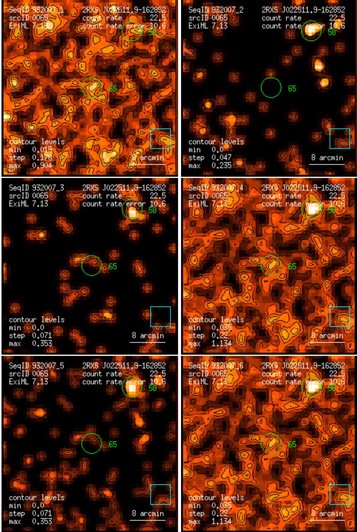
Figure 65: RASS 932007: detection 0065: band rate images, Gaussian filter: (1) PSPC channels 11 – 41, (2) 52 – 90, (3) 91 – 201, (4) 11 – 235, (5) 52 – 201, (6) 11 – 201. Broad band rates in counts/ks. Band rate contour levels in counts/ks/arcmin 2 .
