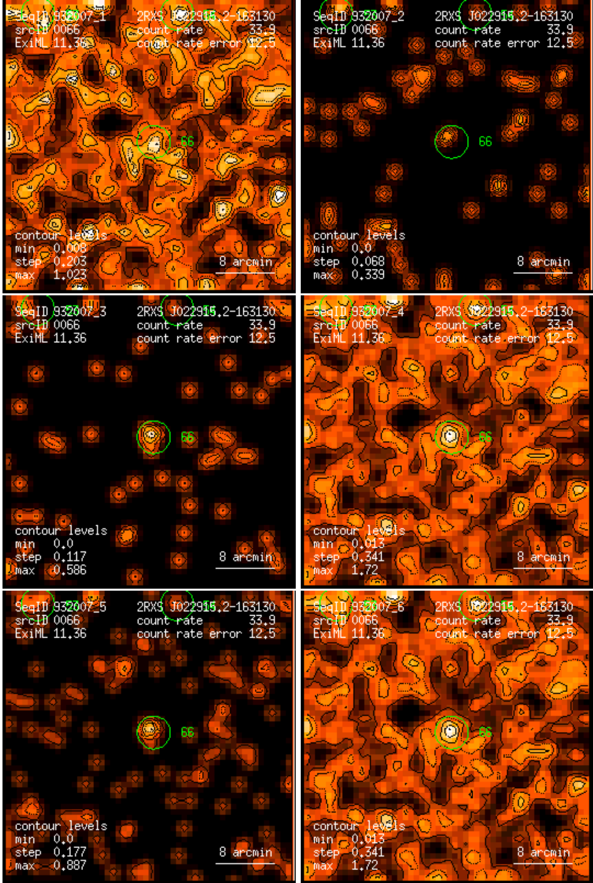
Figure 66: RASS 932007: detection 0066: band rate images, Gaussian filter: (1) PSPC channels 11 – 41, (2) 52 – 90, (3) 91 – 201, (4) 11 – 235, (5) 52 – 201, (6) 11 – 201. Broad band rates in counts/ks. Band rate contour levels in counts/ks/arcmin 2 .
