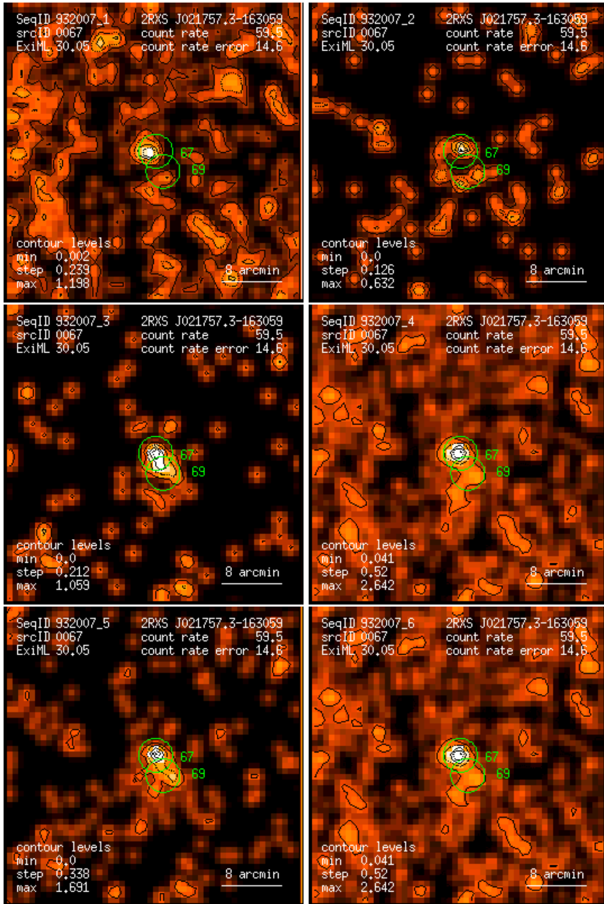
Figure 67: RASS 932007: detection 0067: band rate images, Gaussian filter: (1) PSPC channels 11 – 41, (2) 52 – 90, (3) 91 – 201, (4) 11 – 235, (5) 52 – 201, (6) 11 – 201. Broad band rates in counts/ks. Band rate contour levels in counts/ks/arcmin 2 .
