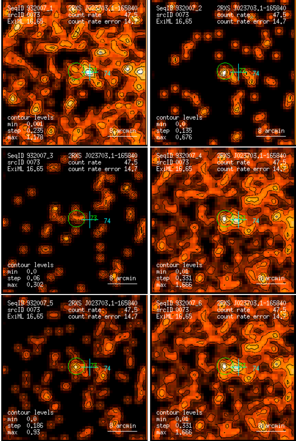
Figure 73: RASS 932007: detection 0073: band rate images, Gaussian filter: (1) PSPC channels 11 – 41, (2) 52 – 90, (3) 91 – 201, (4) 11 – 235, (5) 52 – 201, (6) 11 – 201. Broad band rates in counts/ks. Band rate contour levels in counts/ks/arcmin 2 .
