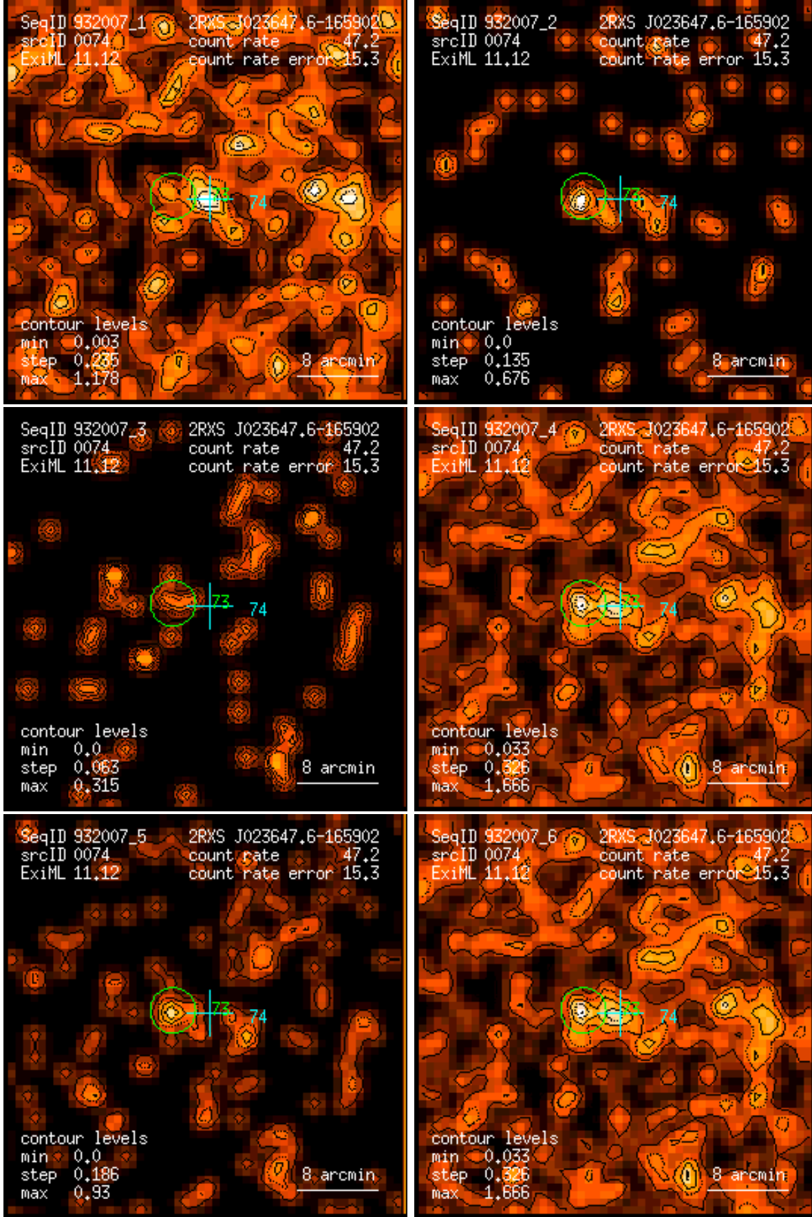
Figure 74: RASS 932007: detection 0074: band rate images, Gaussian filter: (1) PSPC channels 11 – 41, (2) 52 – 90, (3) 91 – 201, (4) 11 – 235, (5) 52 – 201, (6) 11 – 201. Broad band rates in counts/ks. Band rate contour levels in counts/ks/arcmin 2 .
