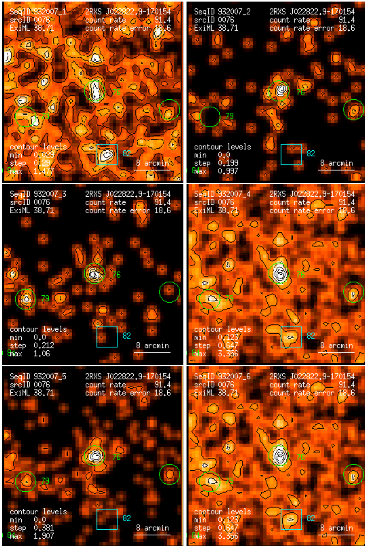
Figure 76: RASS 932007: detection 0076: band rate images, Gaussian filter: (1) PSPC channels 11 – 41, (2) 52 – 90, (3) 91 – 201, (4) 11 – 235, (5) 52 – 201, (6) 11 – 201. Broad band rates in counts/ks. Band rate contour levels in counts/ks/arcmin 2 .
