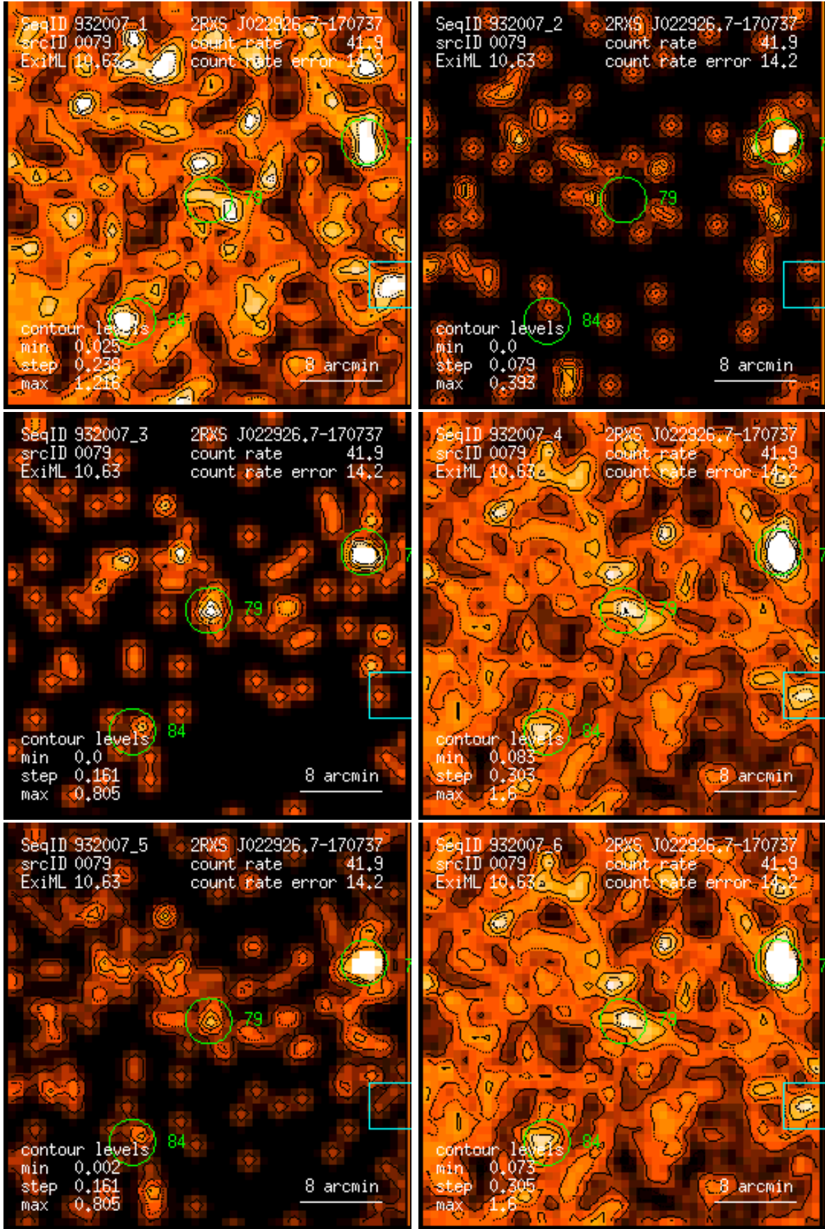
Figure 79: RASS 932007: detection 0079: band rate images, Gaussian filter: (1) PSPC channels 11 – 41, (2) 52 – 90, (3) 91 – 201, (4) 11 – 235, (5) 52 – 201, (6) 11 – 201. Broad band rates in counts/ks. Band rate contour levels in counts/ks/arcmin 2 .
