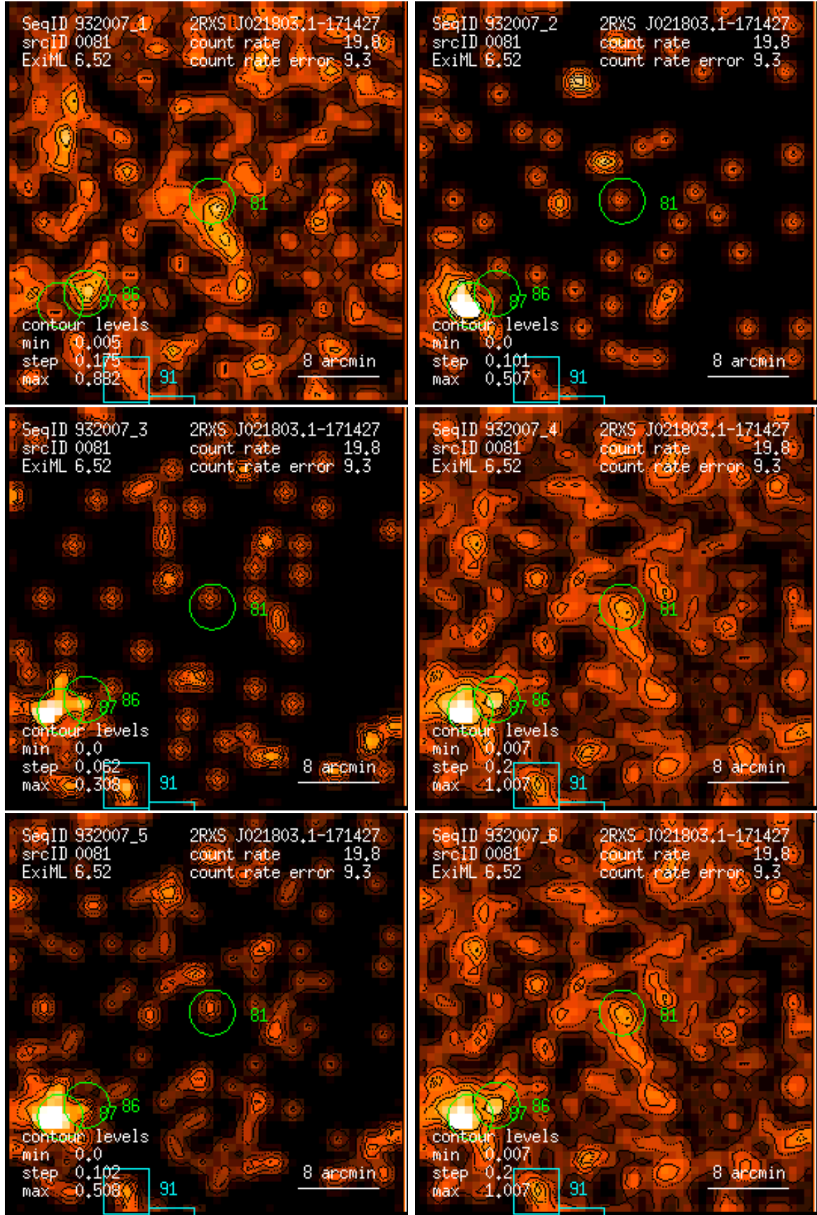
Figure 81: RASS 932007: detection 0081: band rate images, Gaussian filter: (1) PSPC channels 11 – 41, (2) 52 – 90, (3) 91 – 201, (4) 11 – 235, (5) 52 – 201, (6) 11 – 201. Broad band rates in counts/ks. Band rate contour levels in counts/ks/arcmin 2 .
