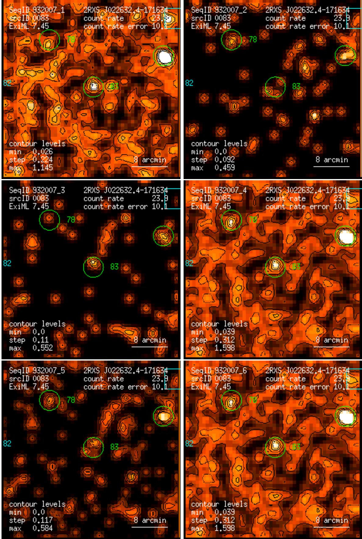
Figure 83: RASS 932007: detection 0083: band rate images, Gaussian filter: (1) PSPC channels 11 – 41, (2) 52 – 90, (3) 91 – 201, (4) 11 – 235, (5) 52 – 201, (6) 11 – 201. Broad band rates in counts/ks. Band rate contour levels in counts/ks/arcmin 2 .
