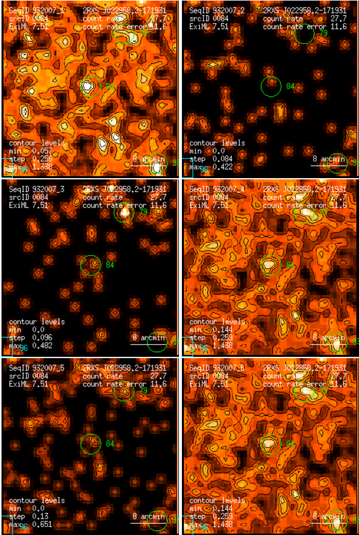
Figure 84: RASS 932007: detection 0084: band rate images, Gaussian filter: (1) PSPC channels 11 – 41, (2) 52 – 90, (3) 91 – 201, (4) 11 – 235, (5) 52 – 201, (6) 11 – 201. Broad band rates in counts/ks. Band rate contour levels in counts/ks/arcmin 2 .
