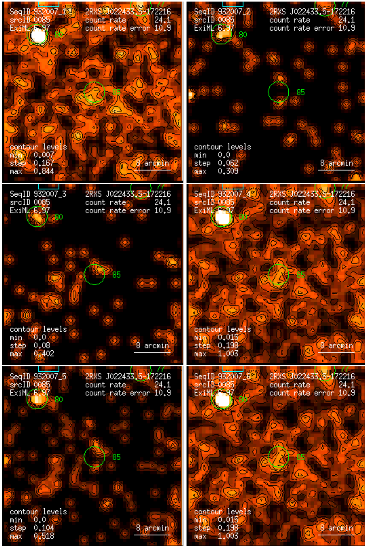
Figure 85: RASS 932007: detection 0085: band rate images, Gaussian filter: (1) PSPC channels 11 – 41, (2) 52 – 90, (3) 91 – 201, (4) 11 – 235, (5) 52 – 201, (6) 11 – 201. Broad band rates in counts/ks. Band rate contour levels in counts/ks/arcmin 2 .
