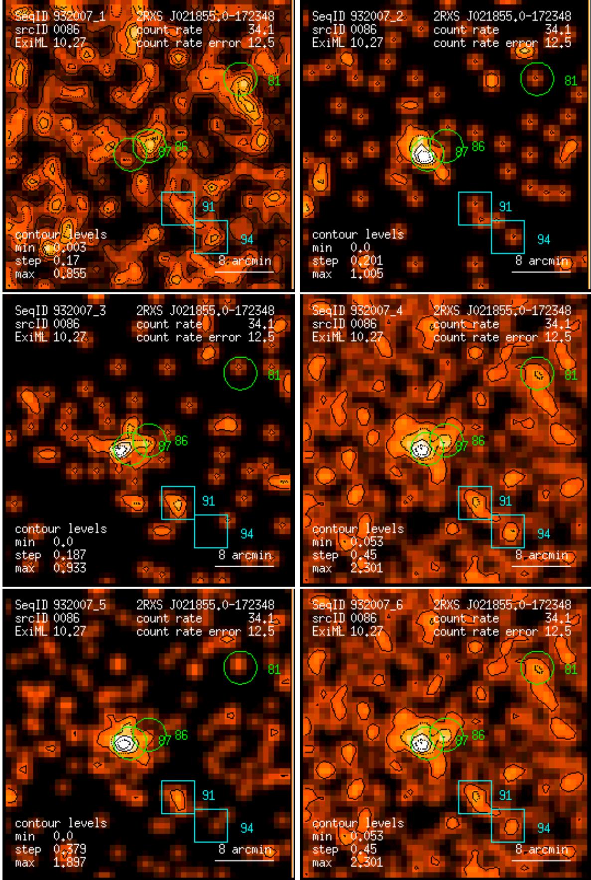
Figure 86: RASS 932007: detection 0086: band rate images, Gaussian filter: (1) PSPC channels 11 – 41, (2) 52 – 90, (3) 91 – 201, (4) 11 – 235, (5) 52 – 201, (6) 11 – 201. Broad band rates in counts/ks. Band rate contour levels in counts/ks/arcmin 2 .
